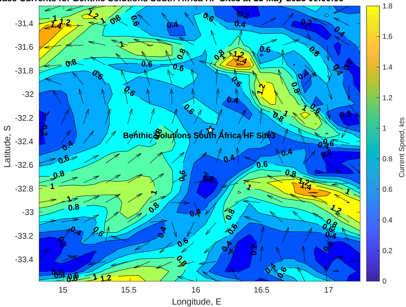
Surface Currents for Benthic Solutions South Africa HF Site3 at 11-May-2025 00:00:00
