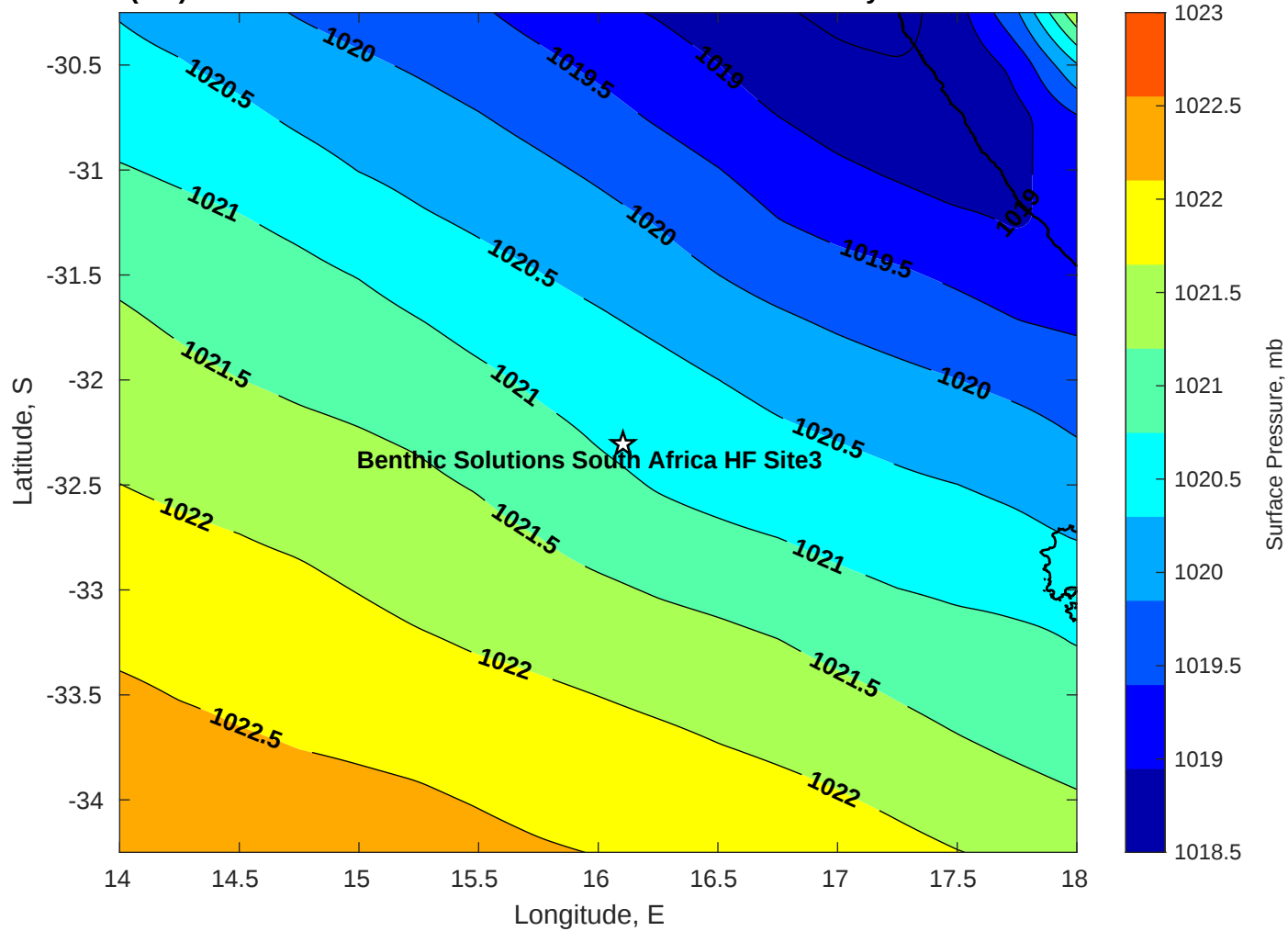
Surface Pressure (mb) for Benthic Solutions South Africa HF Site3 at 14-May-2025 00:00:00
