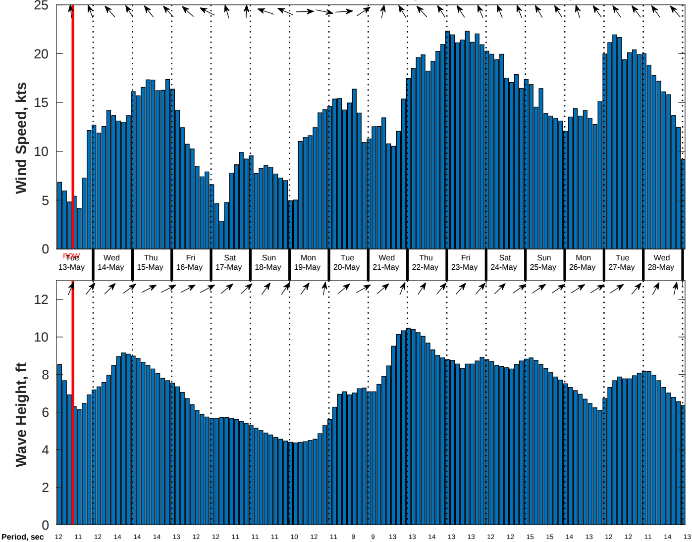
Wind & Wave Forecast for Benthic Solutions South Africa HF Site3 from 12-May-2025 02:00:00 to 28-May-2025 02:00:00
