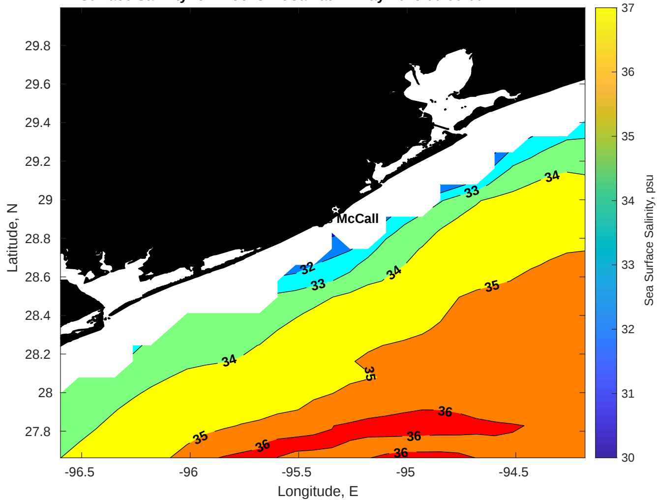
Surface Salinity for Brooks McCall at 11-May-2025 00:00:00
