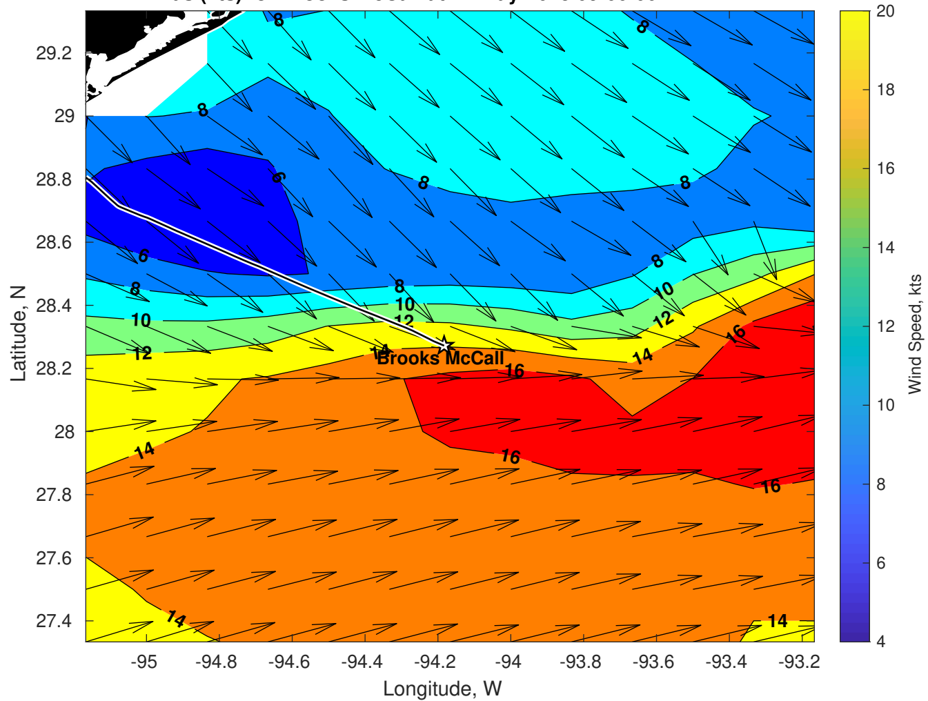
Winds (kts) for Brooks McCall at 12-May-2025 09:00:00
