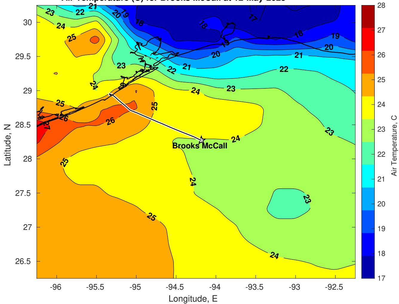
Air Temperature (C) for Brooks McCall at 12-May-2025
