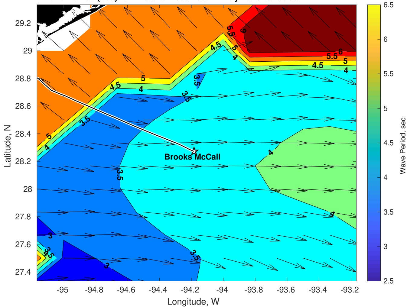
Wave Period (sec) for Brooks McCall at 12-May-2025 09:00:00
