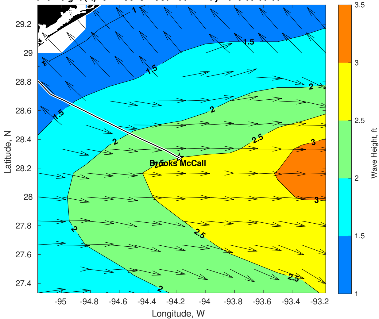
Wave Height (ft) for Brooks McCall at 12-May-2025 09:00:00
