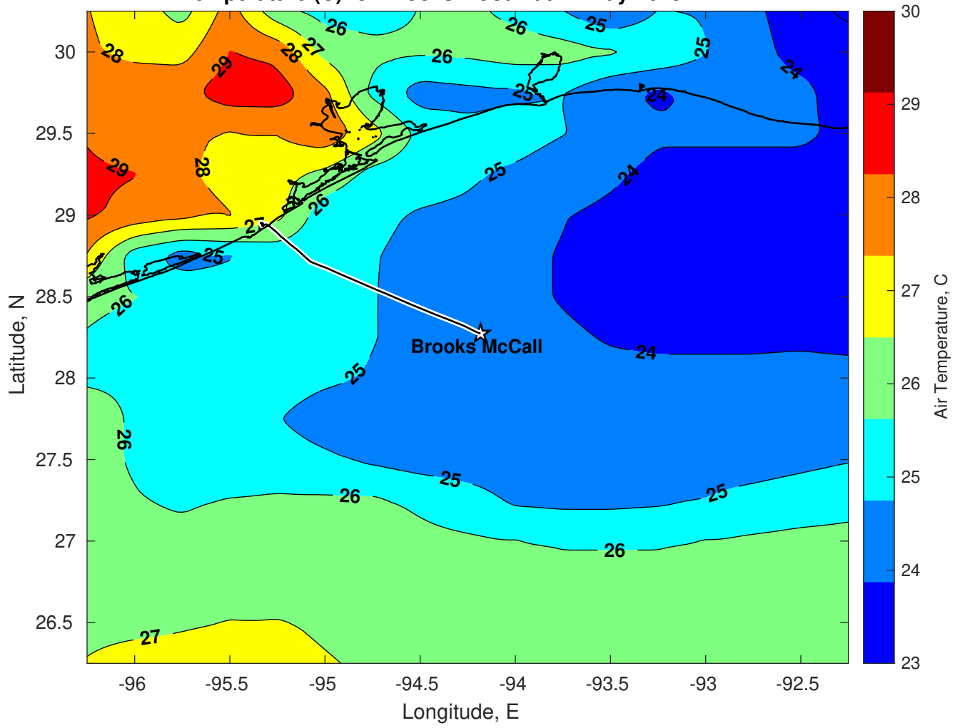
Air Temperature (C) for Brooks McCall at 12-May-2025
