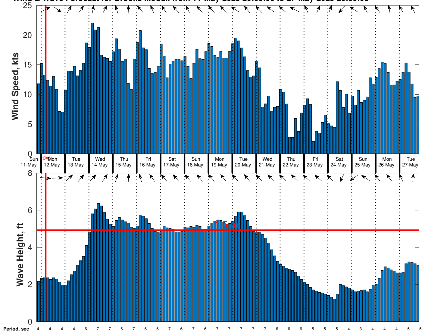
Wind & Wave Forecast for Brooks McCall from 11-May-2025 20:00:00 to 27-May-2025 20:00:00
