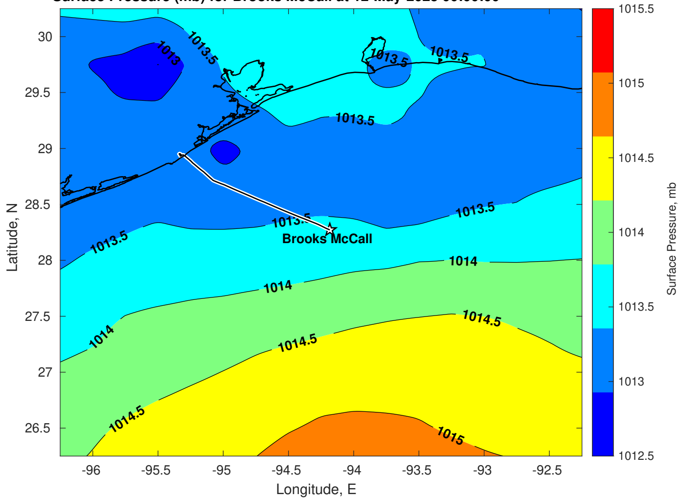
Surface Pressure (mb) for Brooks McCall at 12-May-2025 00:00:00
