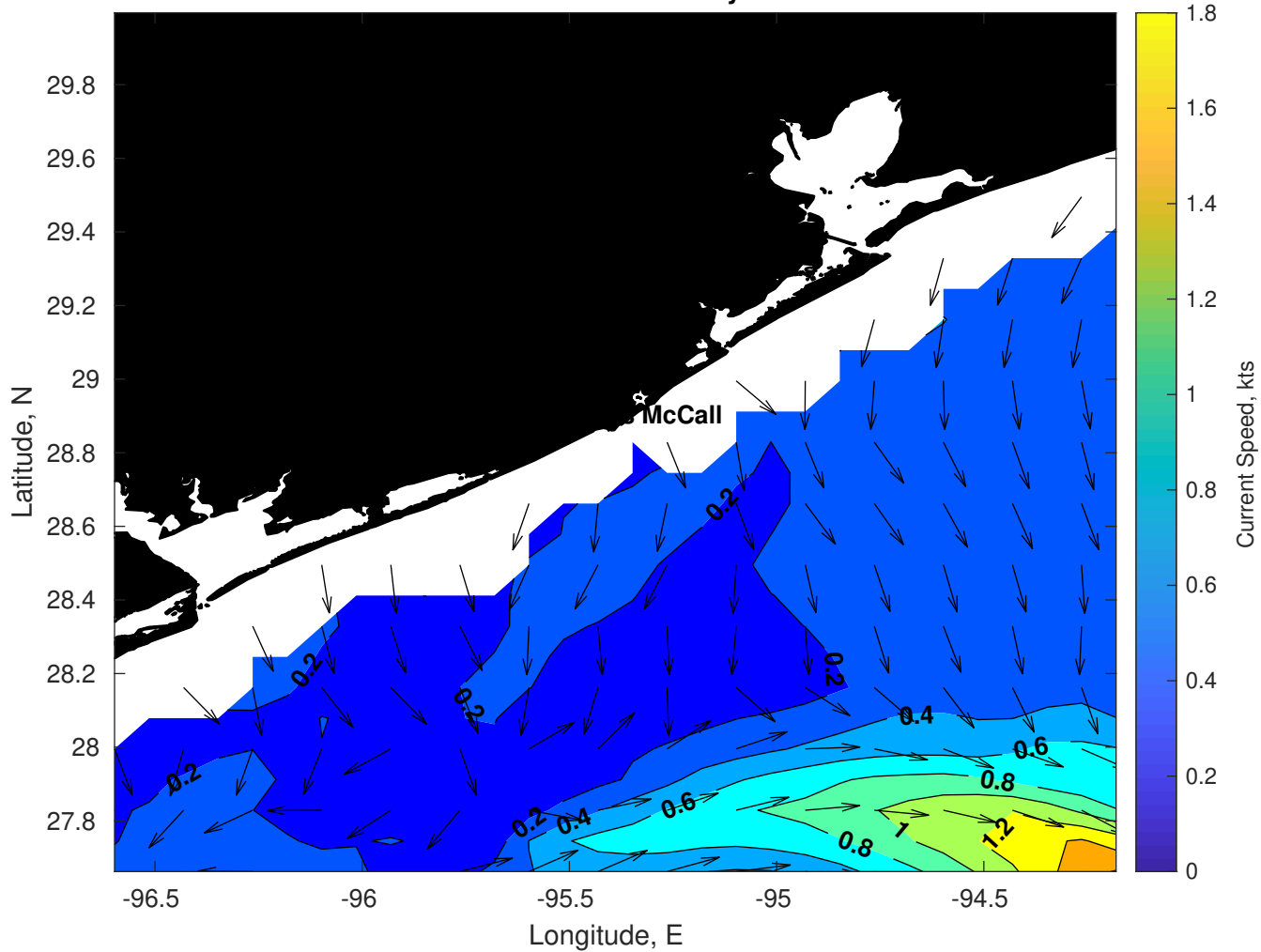
Surface Currents for Brooks McCall at 11-May-2025 00:00:00
