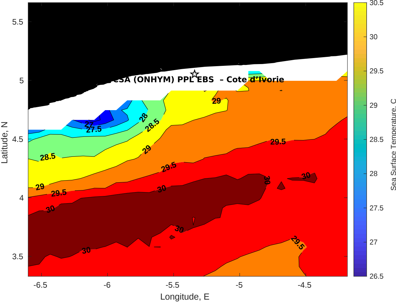
SST for CSA (ONHYM) PPL EBS - Cote d'Ivoire at 11-May-2025 00:00:00
