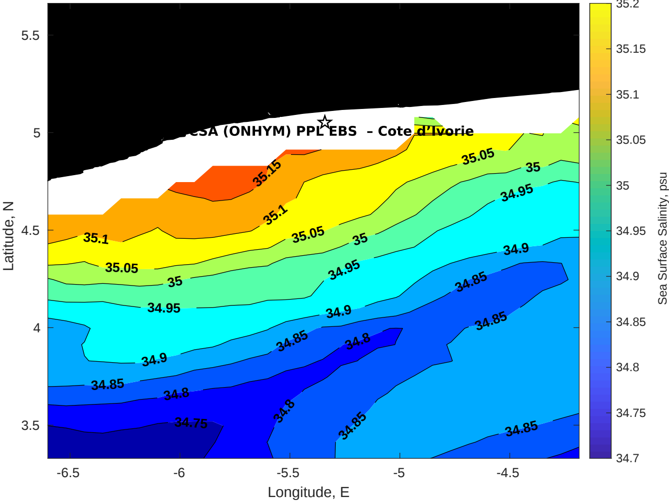
Surface Salinity for CSA (ONHYM) PPL EBS - Cote d'Ivoire at 11-May-2025 00:00:00
