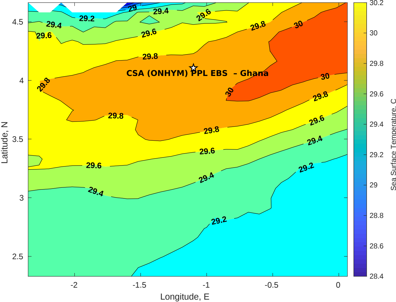
SST for CSA (ONHYM) PPL EBS - Ghana at 11-May-2025 00:00:00
