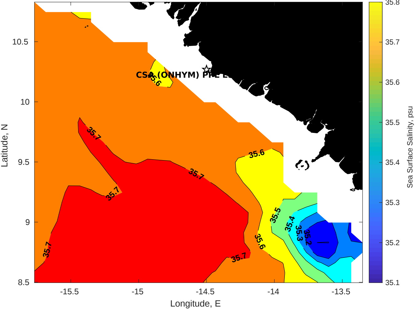
Surface Salinity for CSA (ONHYM) PPL EBS - Guinea at 11-May-2025 00:00:00
