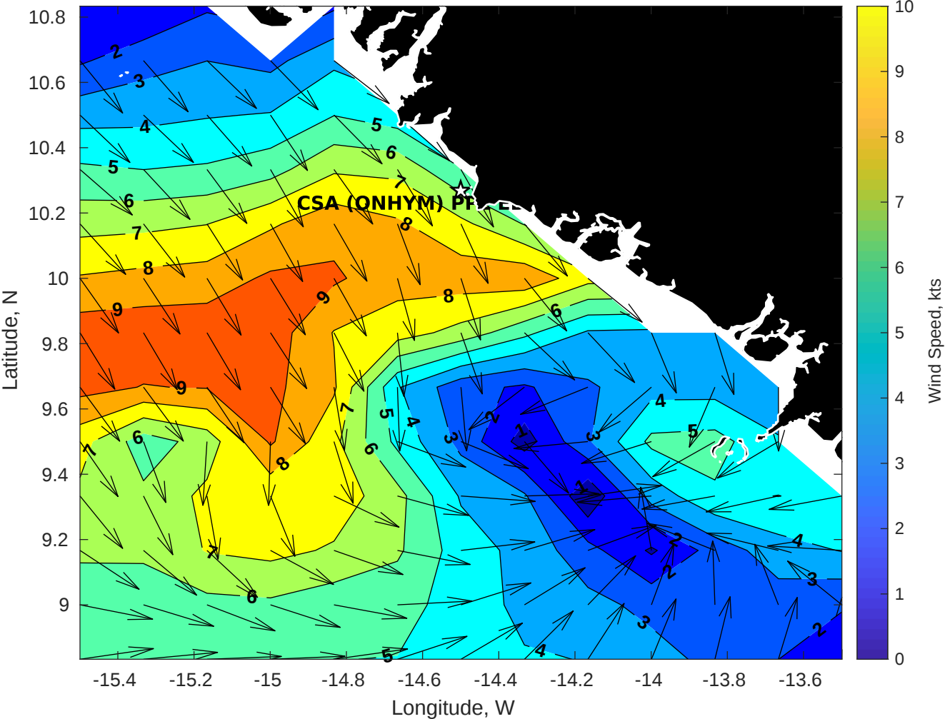
Winds (kts) for CSA (ONHYM) PPL EBS - Guinea at 12-May-2025 09:00:00
