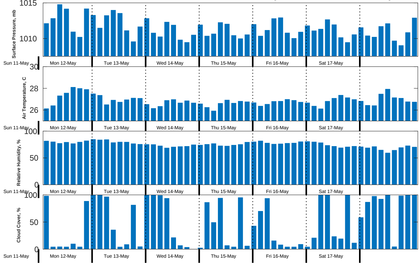
Met Forecast for CSA (ONHYM) PPL EBS - Guinea from 12-May-2025 00:00:00 to 19-May-2025 00:00:00
