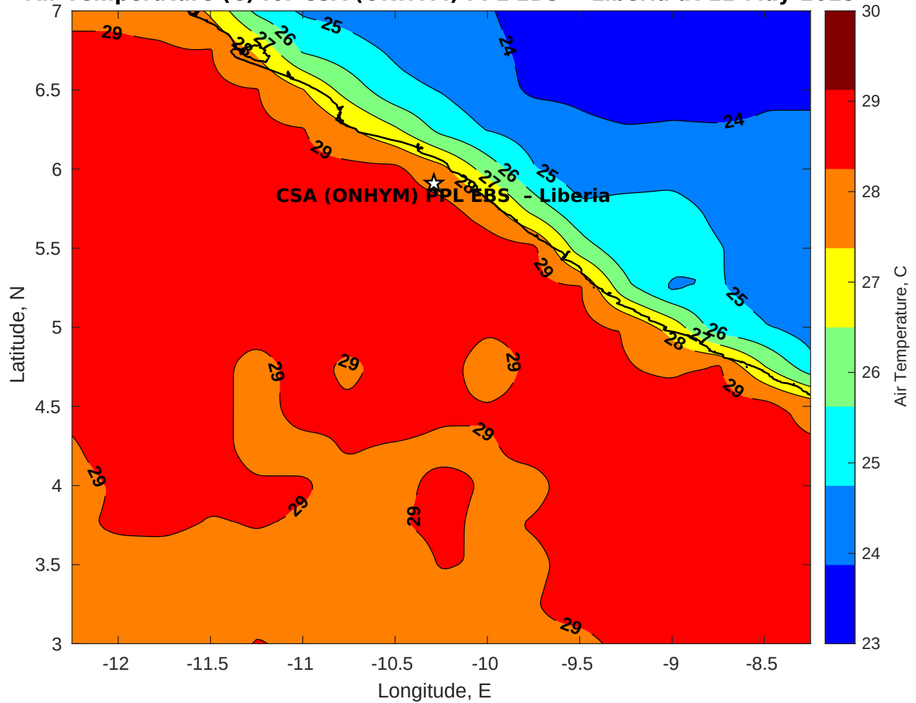
Air Temperature (C) for CSA (ONHYM) PPL EBS - Liberia at 12-May-2025
