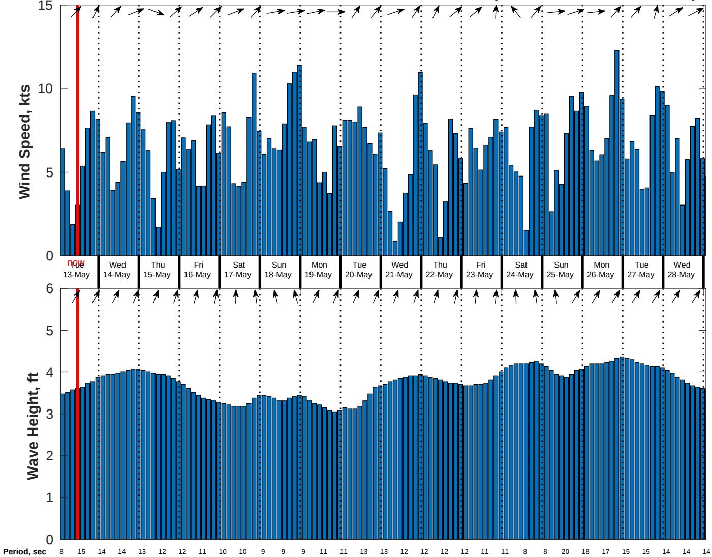
Wind & Wave Forecast for CSA (ONHYM) PPL EBS - Liberia from 12-May-2025 01:00:00 to 28-May-2025 01:00:00
