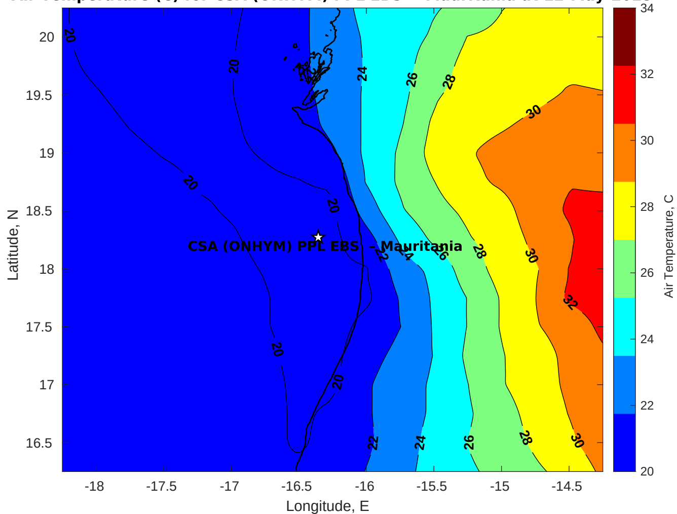
Air Temperature (C) for CSA (ONHYM) PPL EBS - Mauritania at 12-May-2025
