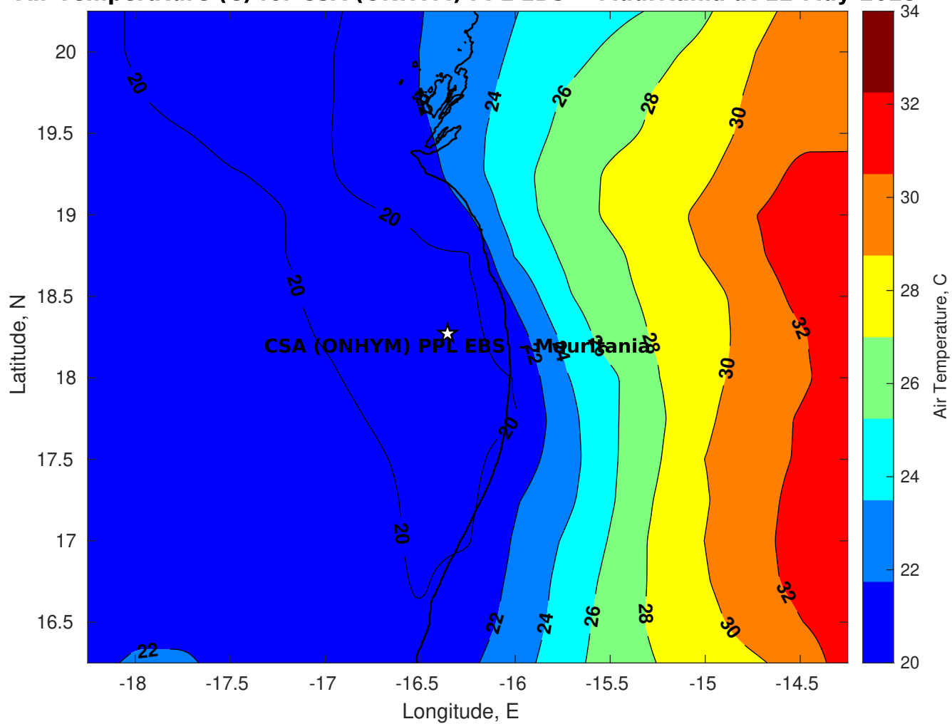
Air Temperature (C) for CSA (ONHYM) PPL EBS - Mauritania at 12-May-2025
