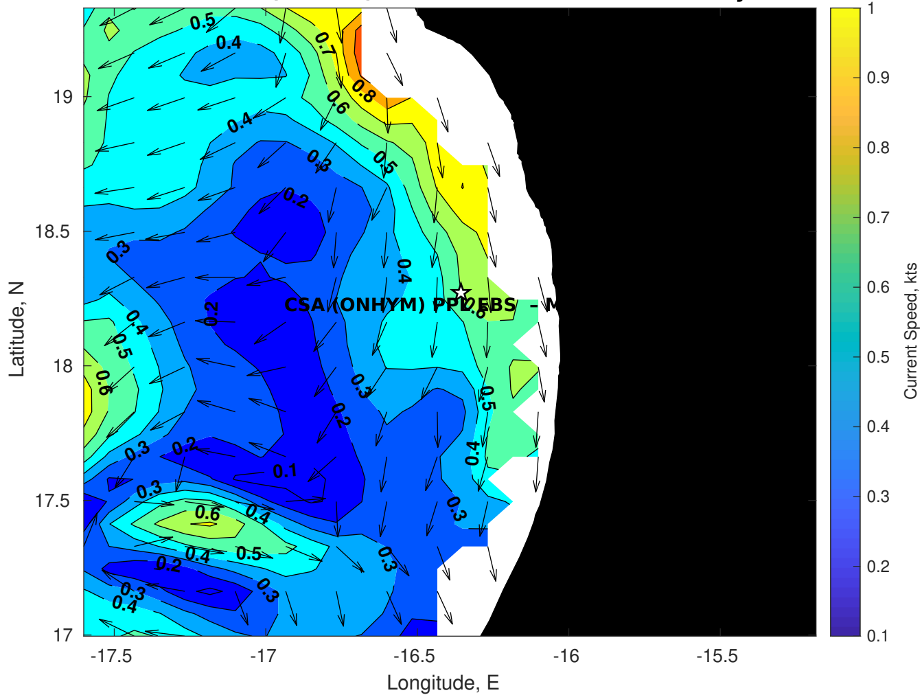
Surface Currents for CSA (ONHYM) PPL EBS - Mauritania at 11-May-2025 00:00:00
