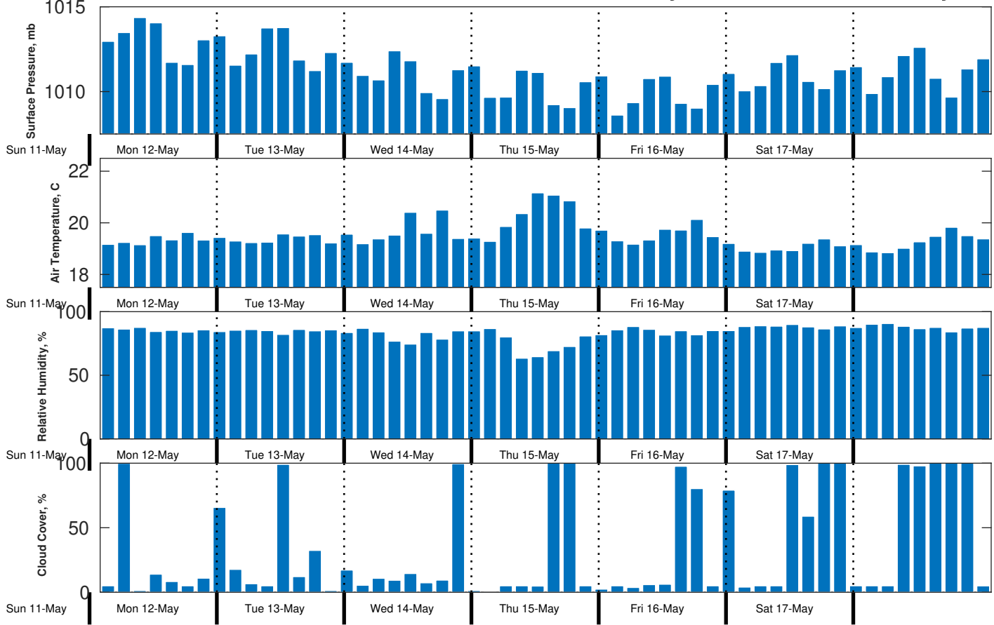
Met Forecast for CSA (ONHYM) PPL EBS - Mauritania from 12-May-2025 00:00:00 to 19-May-2025 00:00:00
