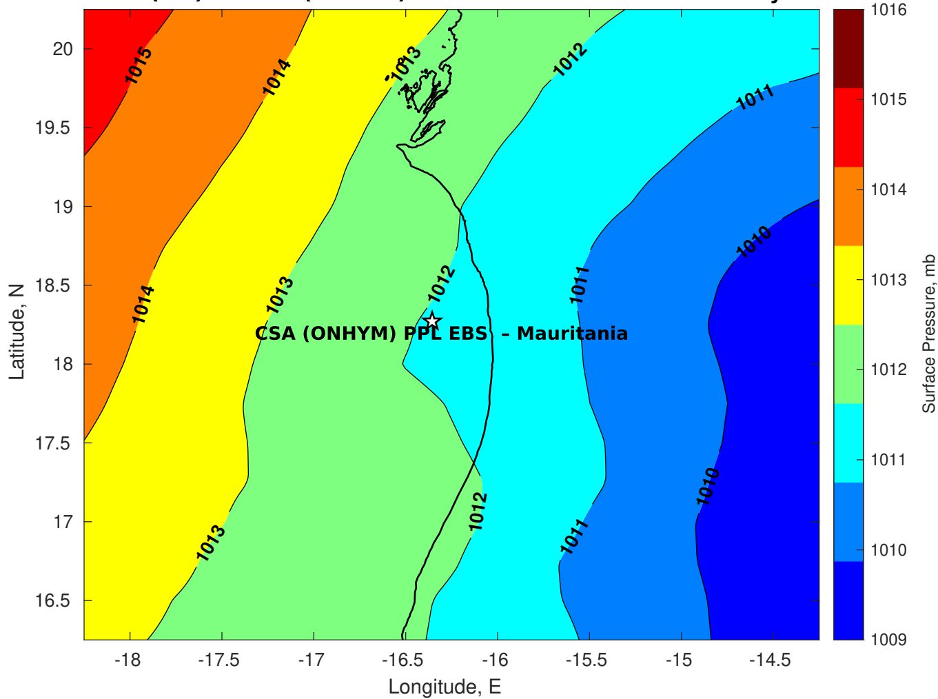
Surface Pressure (mb) for CSA (ONHYM) PPL EBS - Mauritania at 14-May-2025 00:00:00
