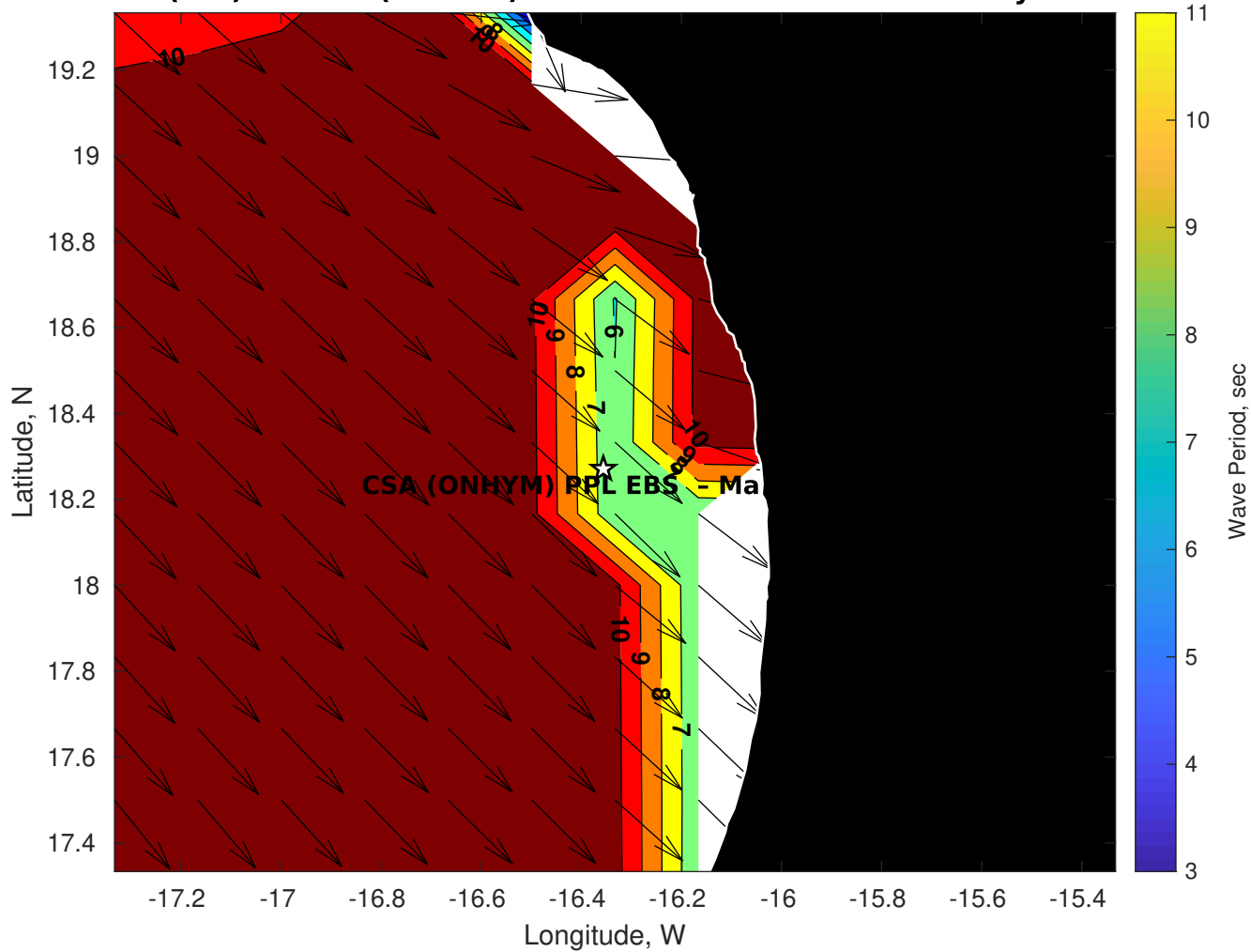
Wave Period (sec) for CSA (ONHYM) PPL EBS - Mauritania at 12-May-2025 09:00:00
