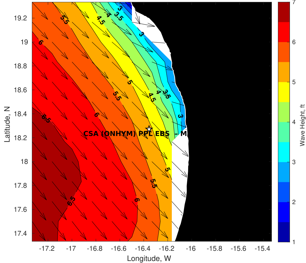
Wave Height (ft) for CSA (ONHYM) PPL EBS - Mauritania at 12-May-2025 09:00:00
