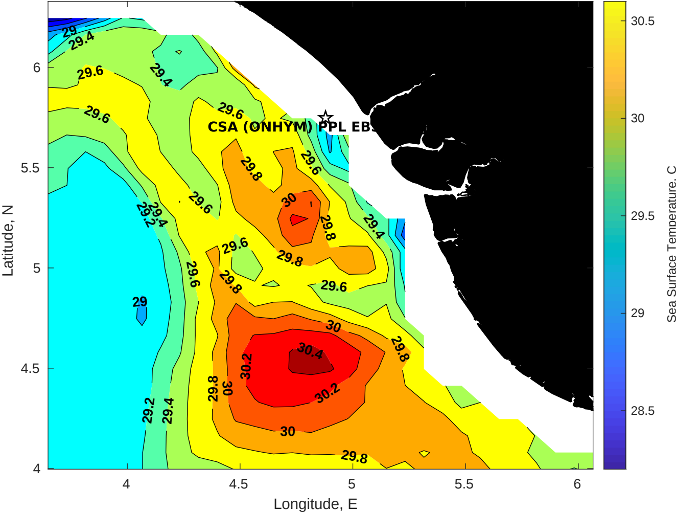
SST for CSA (ONHYM) PPL EBS - Nigeria at 11-May-2025 00:00:00
