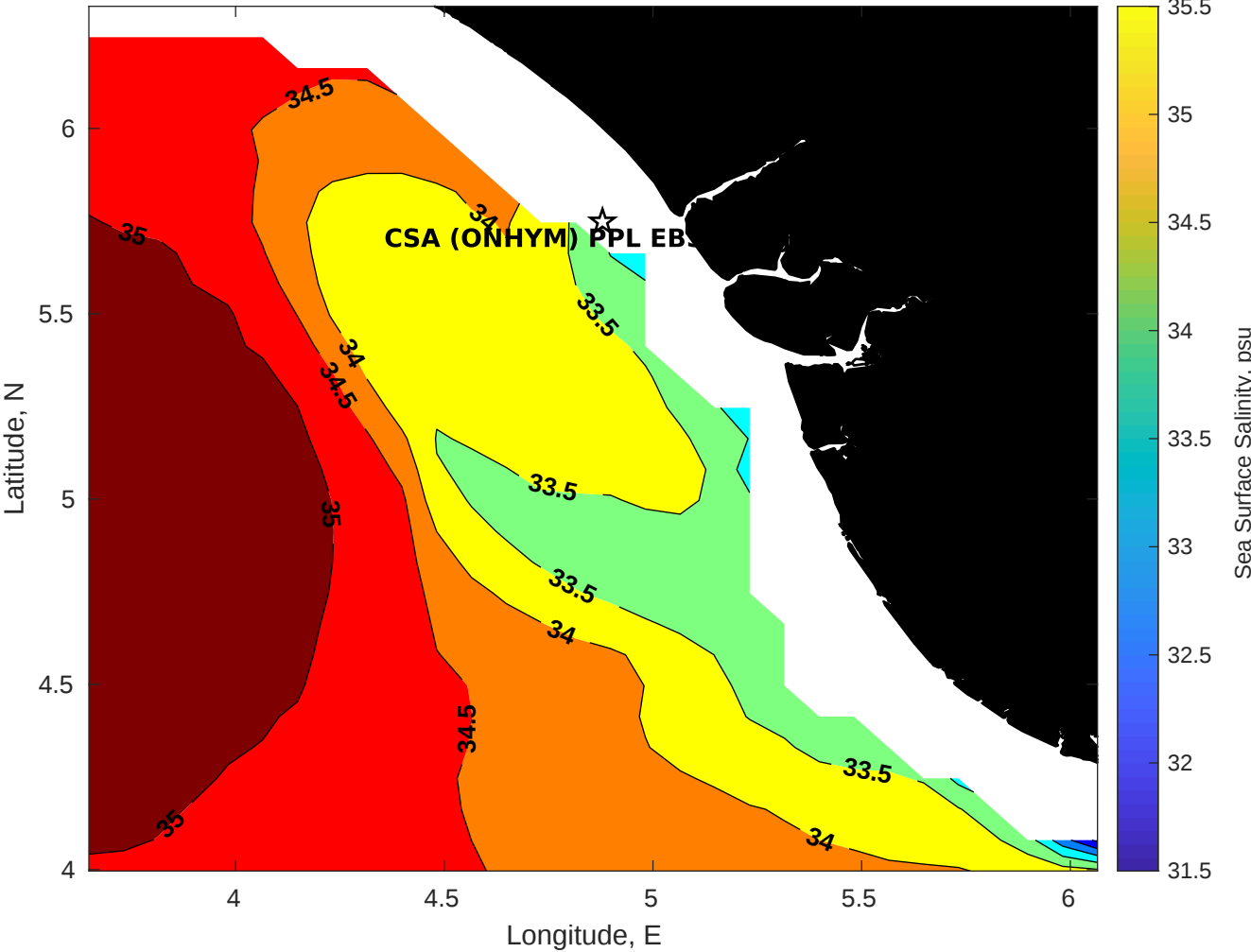
Surface Salinity for CSA (ONHYM) PPL EBS - Nigeria at 11-May-2025 00:00:00
