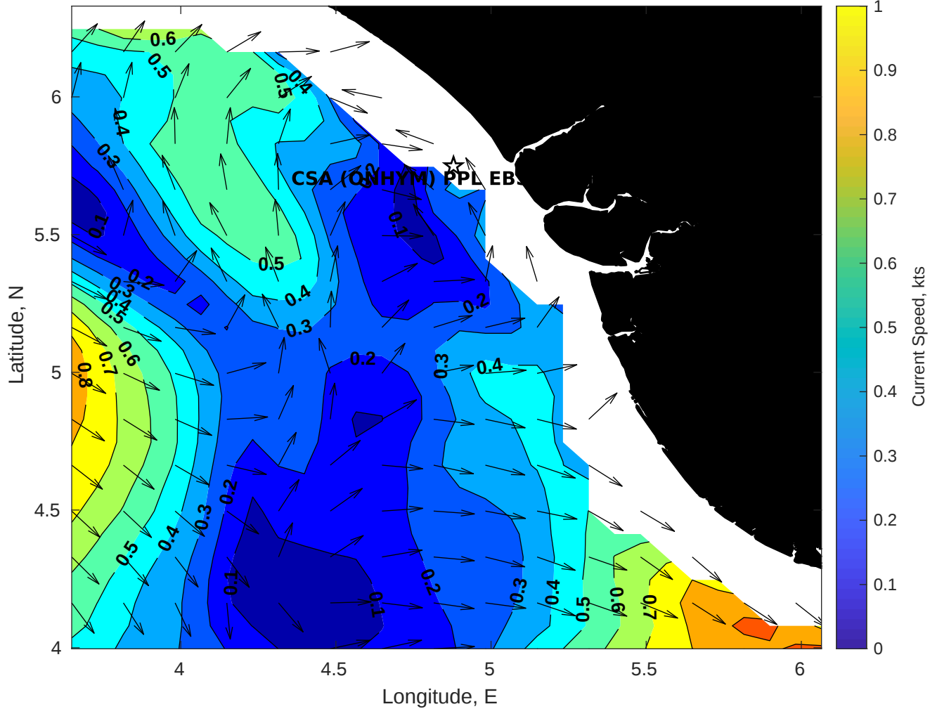
Surface Currents for CSA (ONHYM) PPL EBS - Nigeria at 11-May-2025 00:00:00
