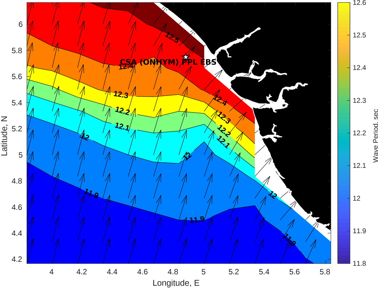
Wave Period (sec) for CSA (ONHYM) PPL EBS - Nigeria at 12-May-2025 09:00:00
