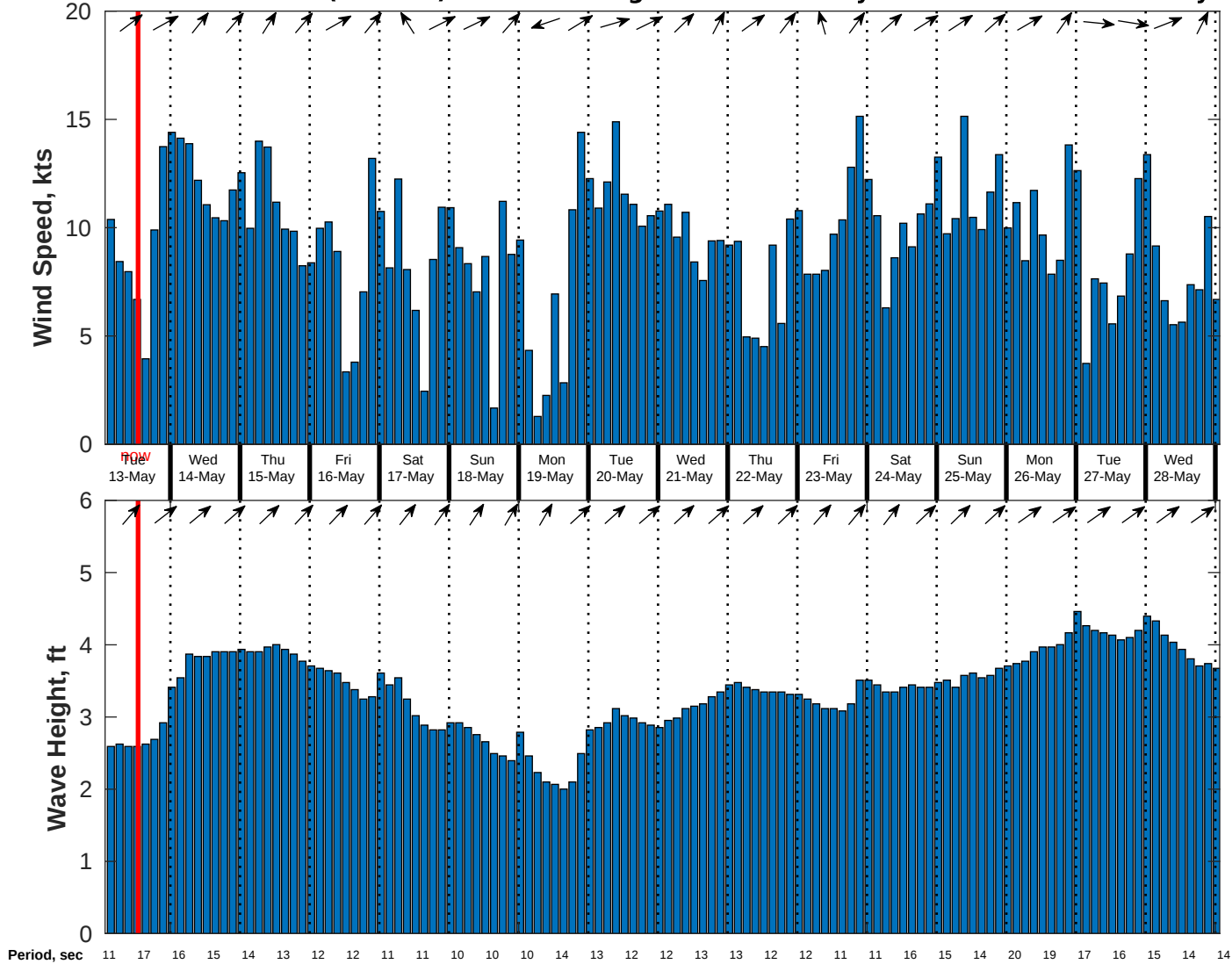
Wind & Wave Forecast for CSA (ONHYM) PPL EBS - Nigeria from 12-May-2025 02:00:00 to 28-May-2025 02:00:00
