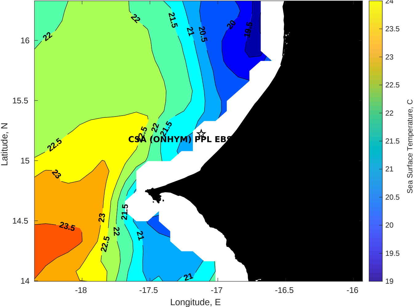
SST for CSA (ONHYM) PPL EBS - Senegal at 11-May-2025 00:00:00
