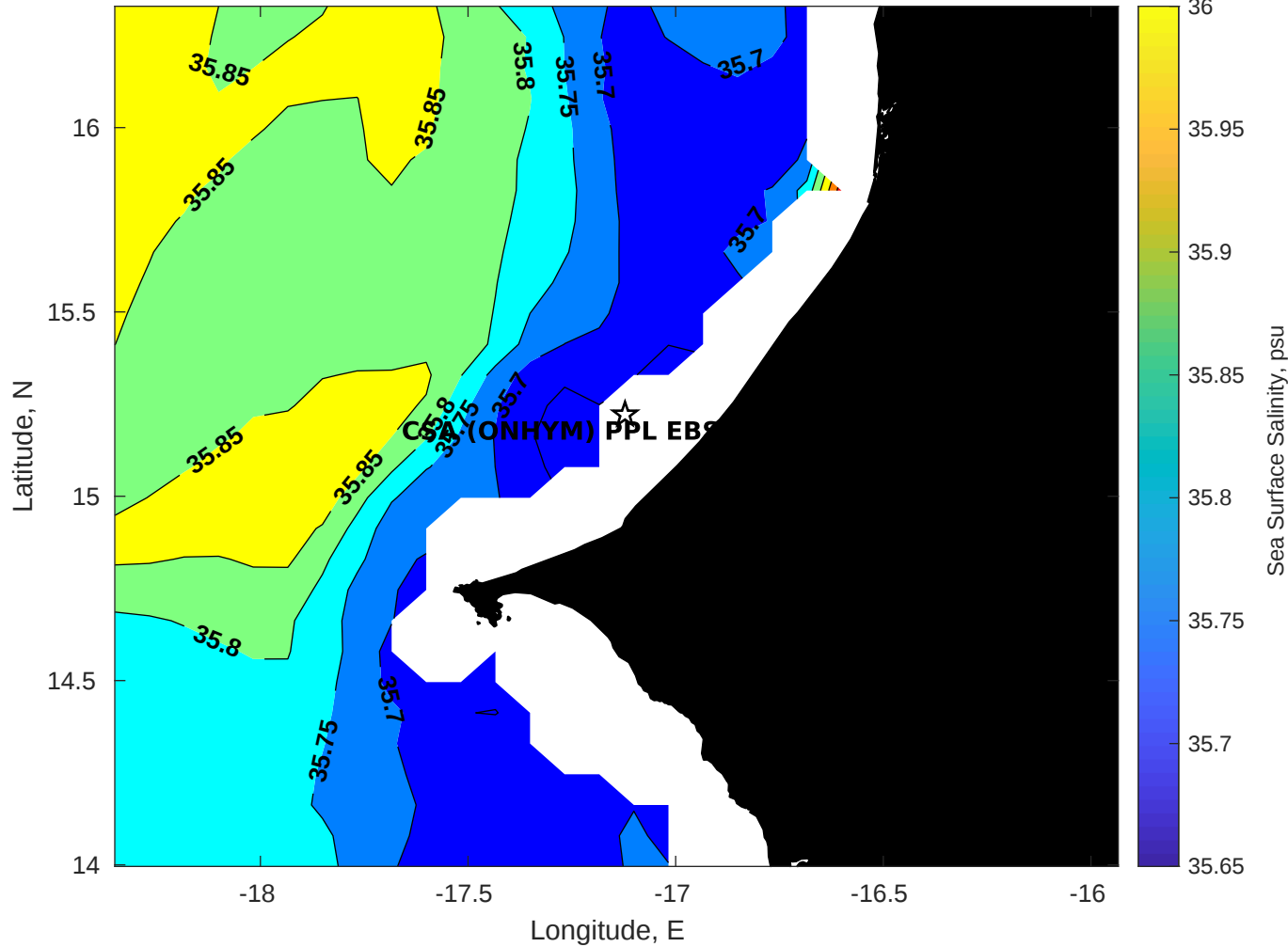
Surface Salinity for CSA (ONHYM) PPL EBS - Senegal at 11-May-2025 00:00:00
