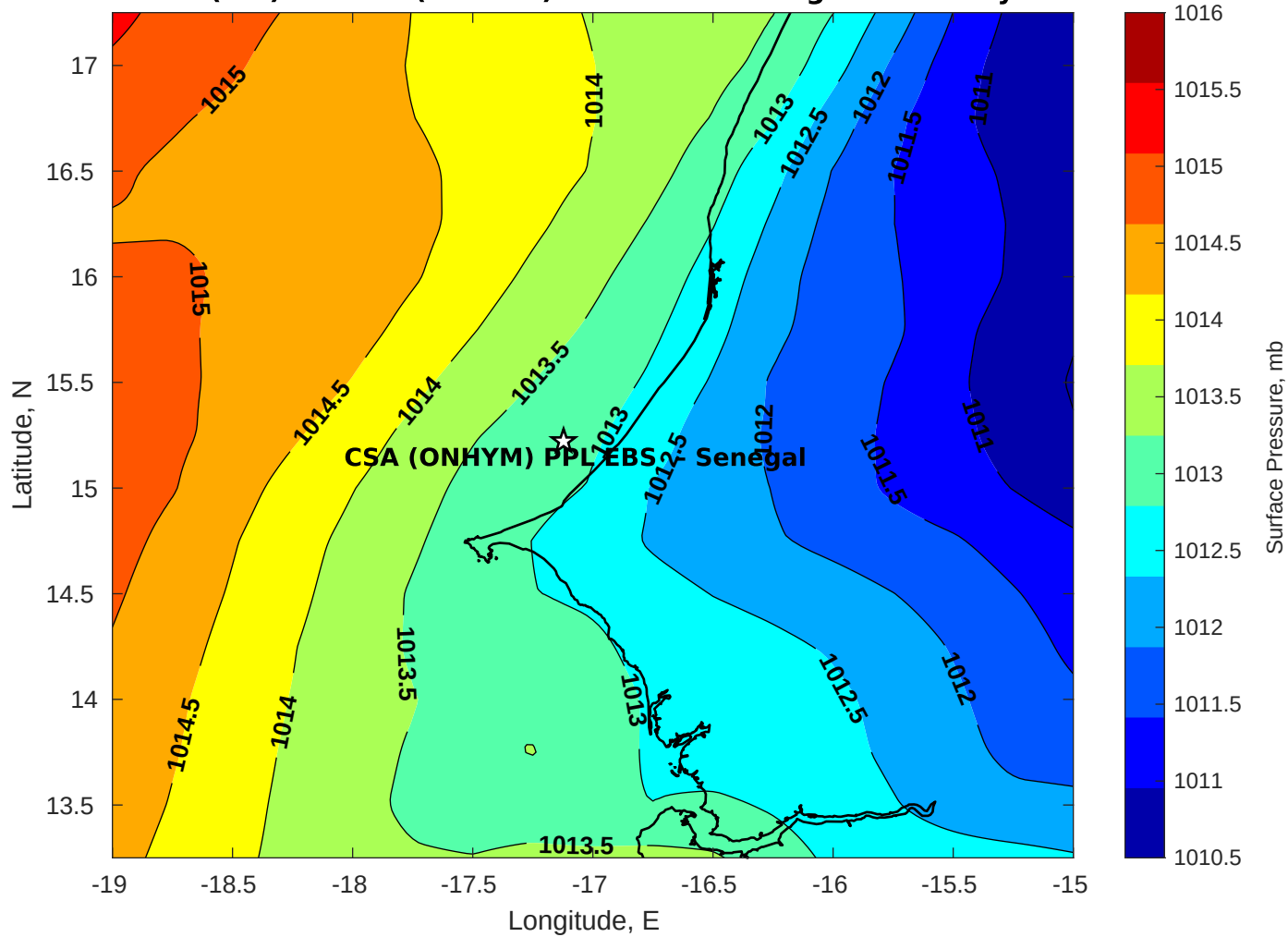
Surface Pressure (mb) for CSA (ONHYM) PPL EBS - Senegal at 13-May-2025 00:00:00
