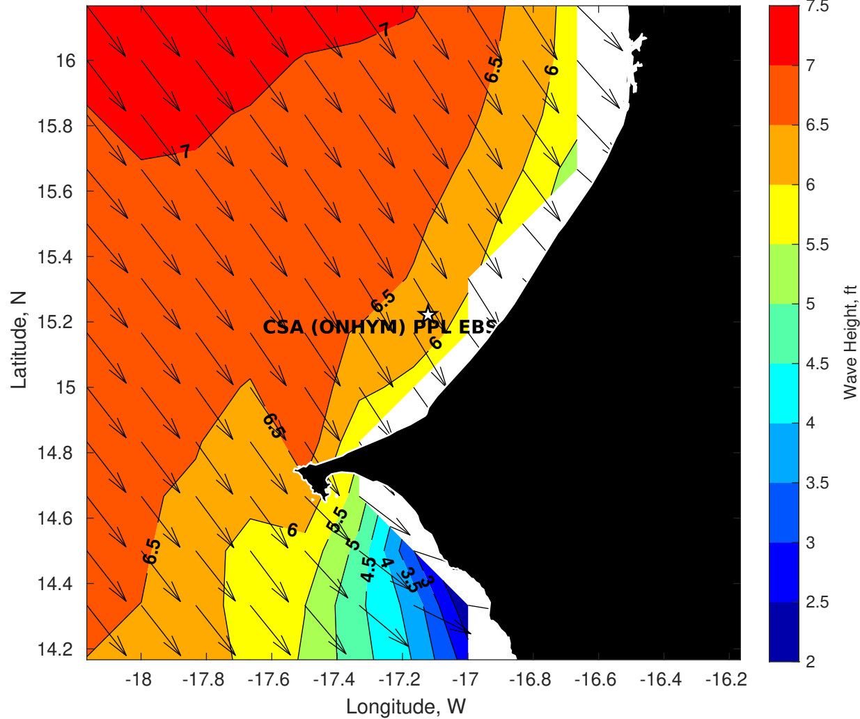
Wave Height (ft) for CSA (ONHYM) PPL EBS - Senegal at 12-May-2025 09:00:00
