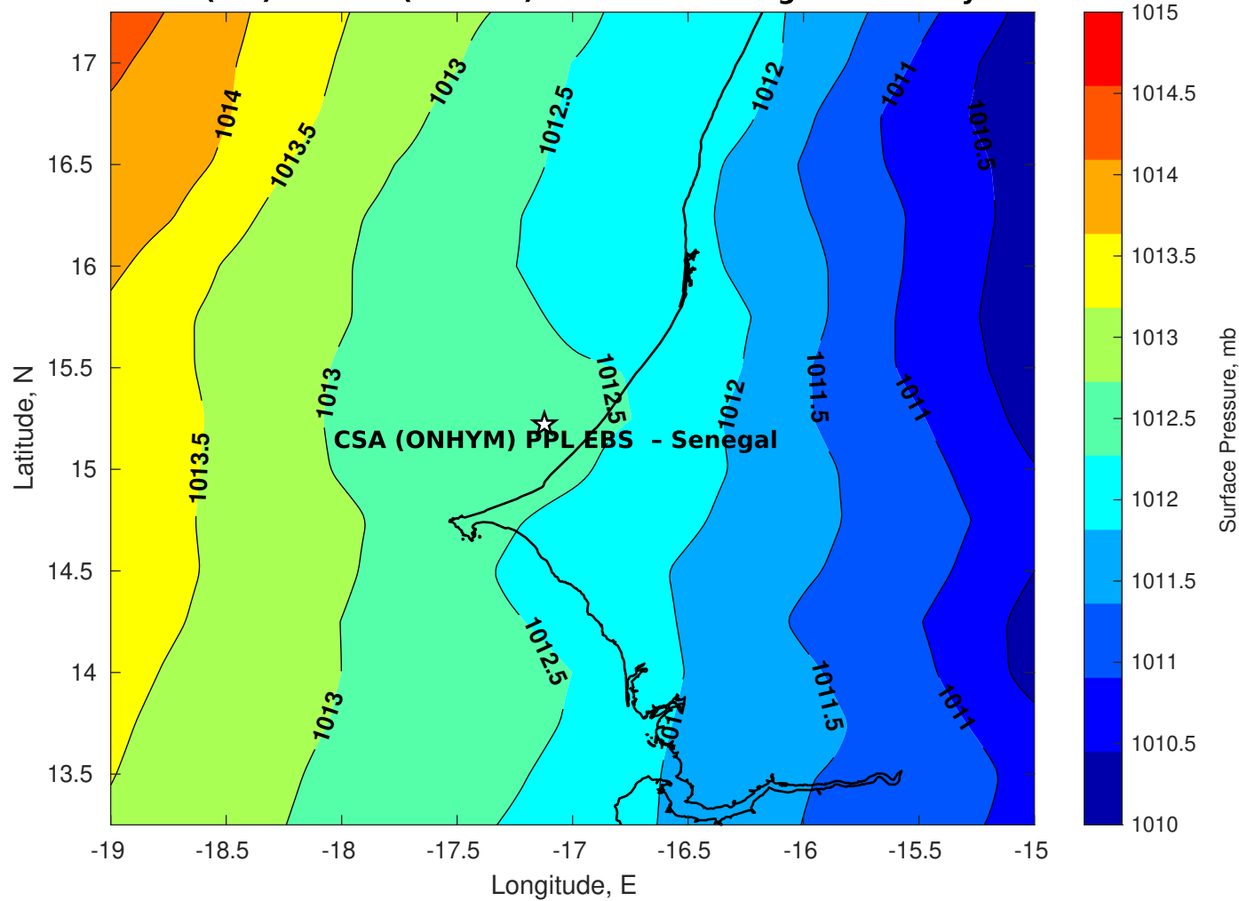
Surface Pressure (mb) for CSA (ONHYM) PPL EBS - Senegal at 14-May-2025 00:00:00
