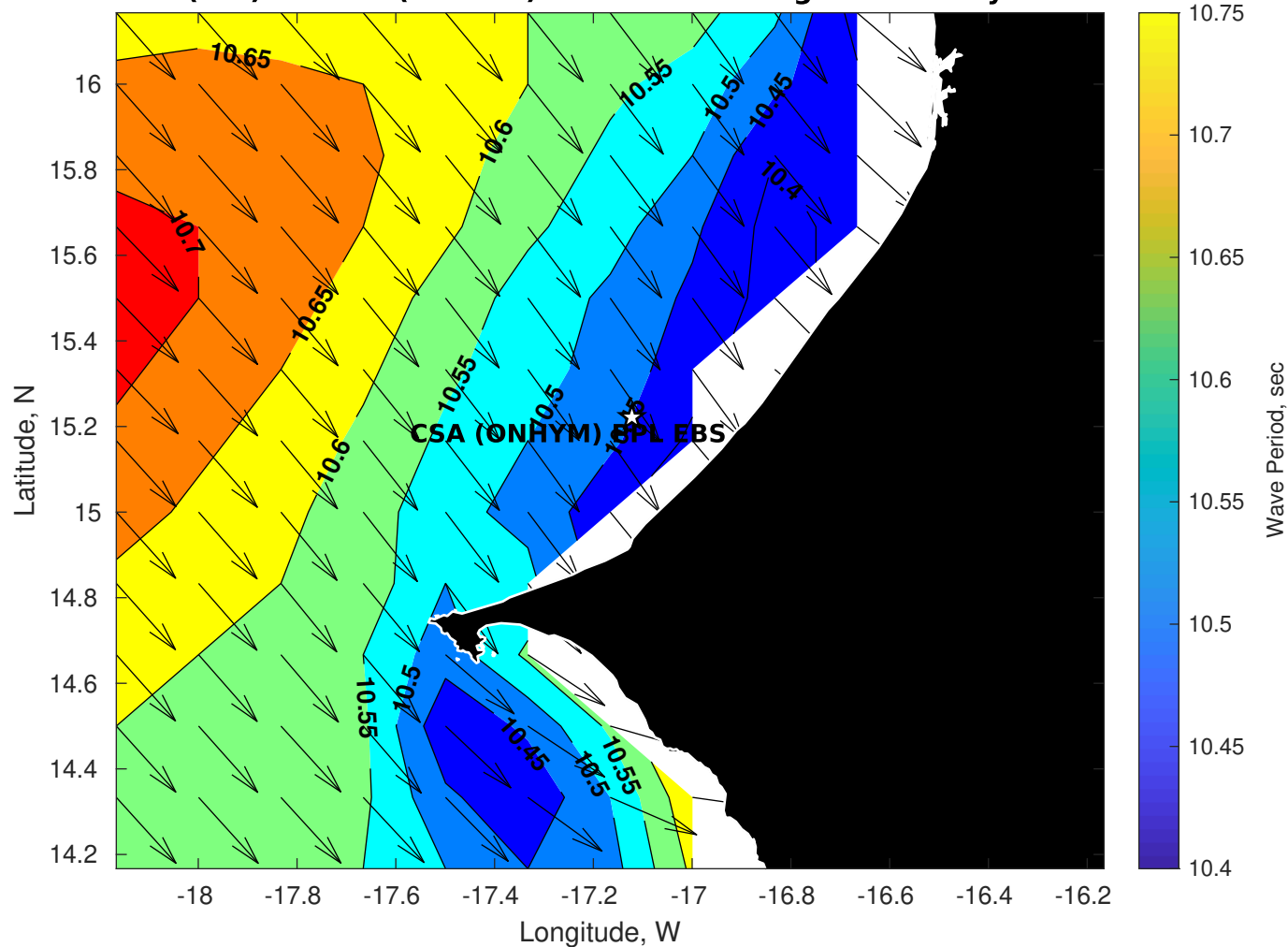
Wave Period (sec) for CSA (ONHYM) PPL EBS - Senegal at 12-May-2025 09:00:00
