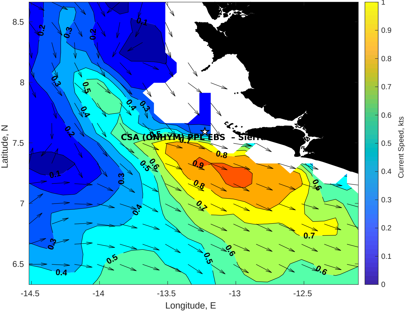
Surface Currents for CSA (ONHYM) PPL EBS - Sierra Leone at 11-May-2025 00:00:00
