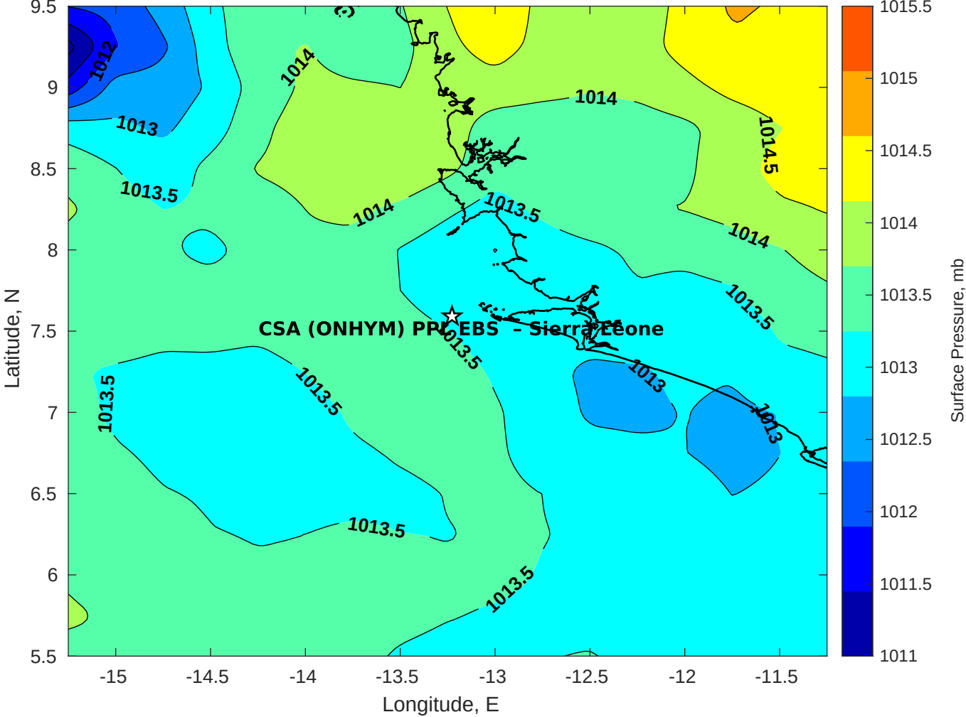
Surface Pressure (mb) for CSA (ONHYM) PPL EBS - Sierra Leone at 12-May-2025 00:00:00
