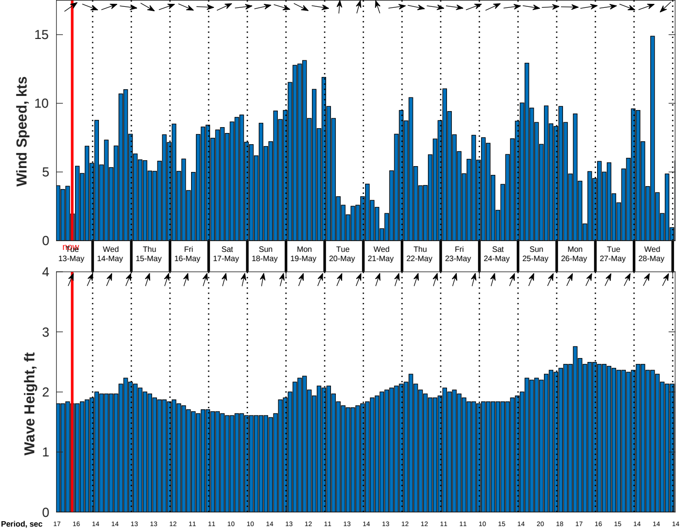
Wind & Wave Forecast for CSA (ONHYM) PPL EBS - Sierra Leone from 12-May-2025 01:00:00 to 28-May-2025 01:00:00
