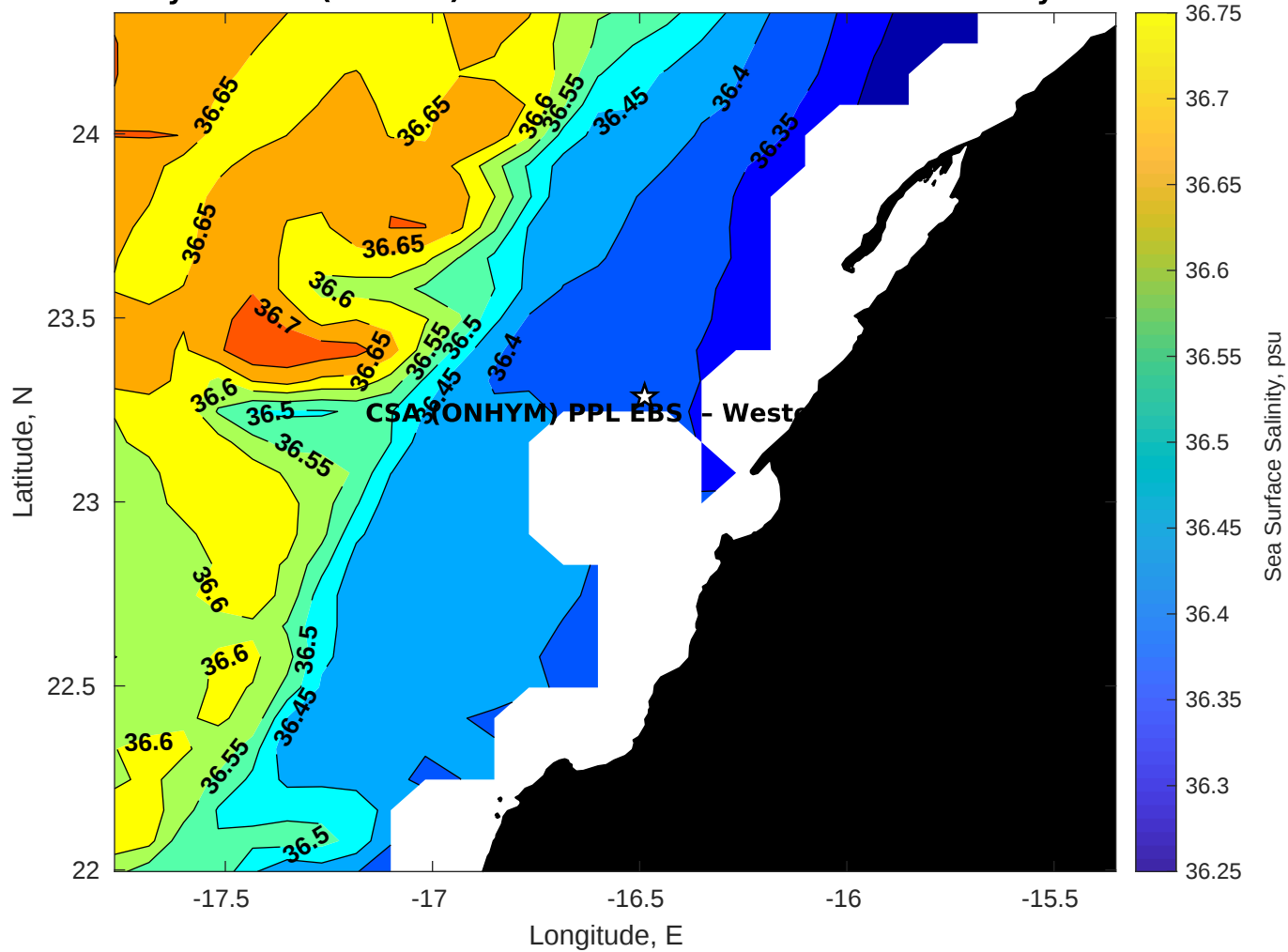
Surface Salinity for CSA (ONHYM) PPL EBS - Western Sahara at 11-May-2025 00:00:00
