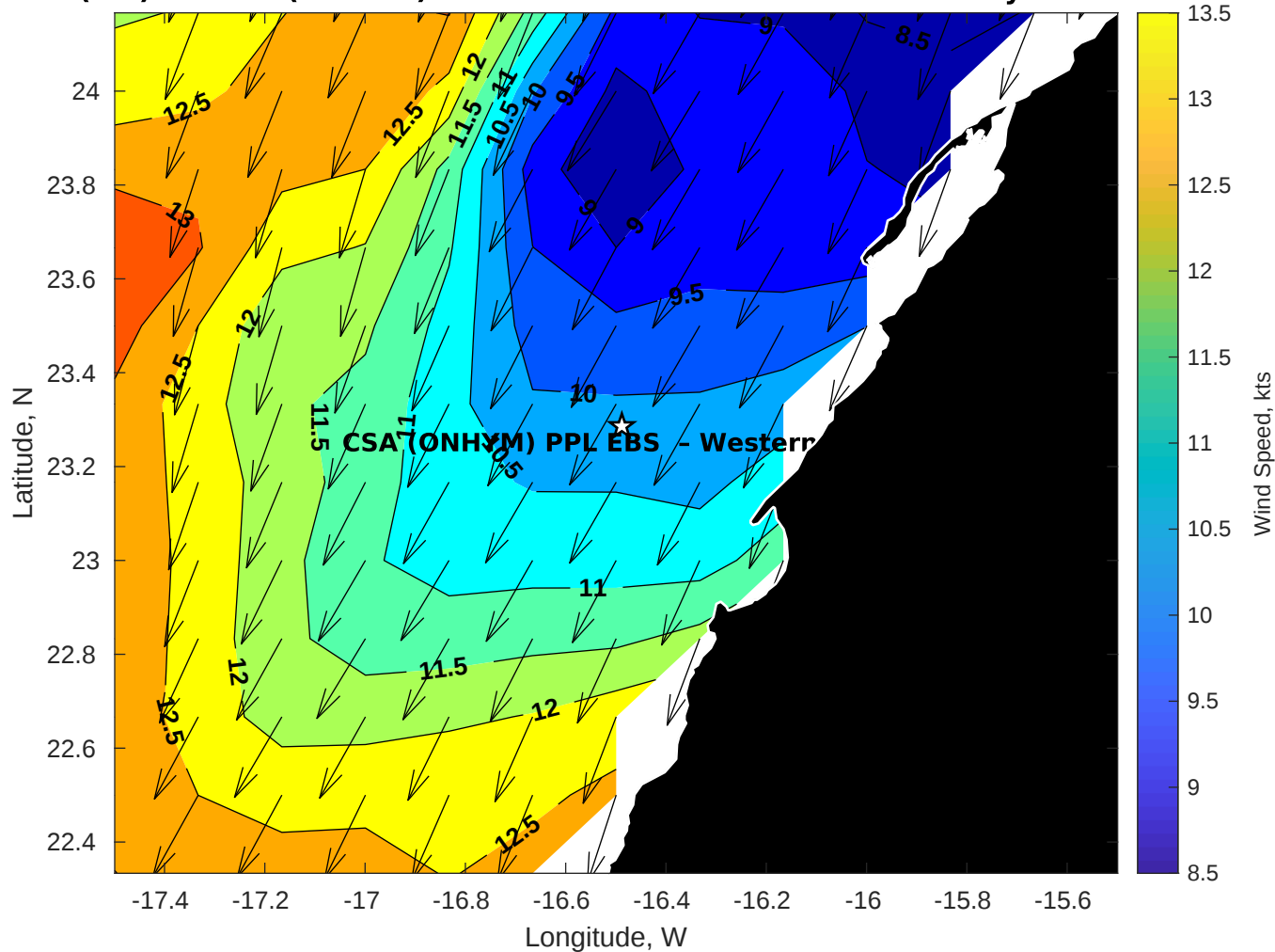
Winds (kts) for CSA (ONHYM) PPL EBS - Western Sahara at 12-May-2025 09:00:00
