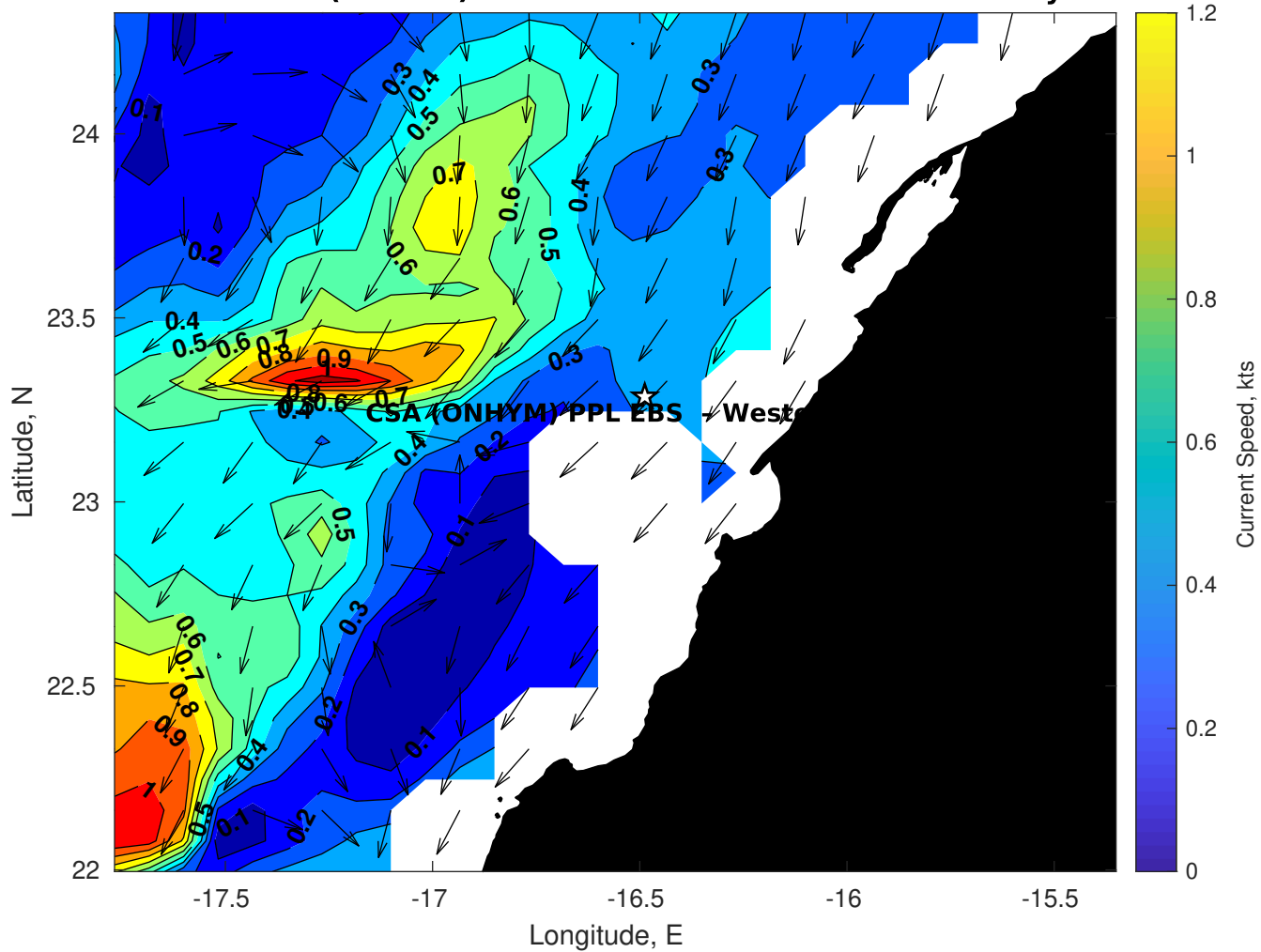
Surface Currents for CSA (ONHYM) PPL EBS - Western Sahara at 11-May-2025 00:00:00
