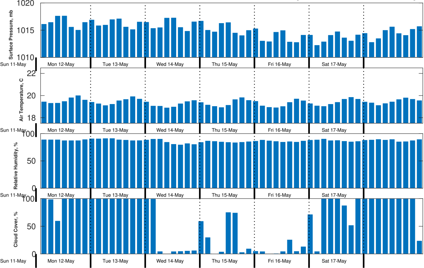
Met Forecast for CSA (ONHYM) PPL EBS - Western Sahara from 12-May-2025 00:00:00 to 19-May-2025 00:00:00
