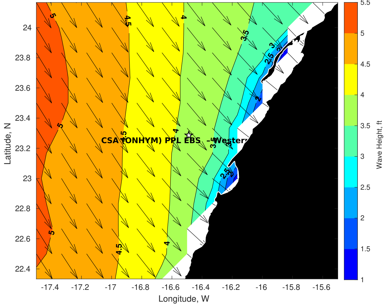
Wave Height (ft) for CSA (ONHYM) PPL EBS - Western Sahara at 12-May-2025 09:00:00
