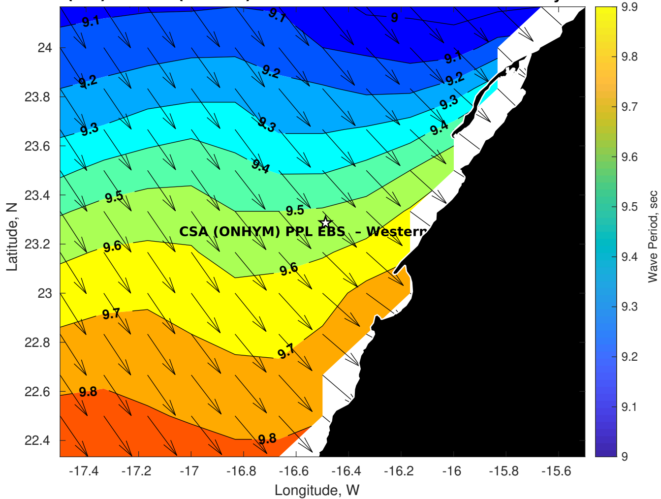
Wave Period (sec) for CSA (ONHYM) PPL EBS - Western Sahara at 12-May-2025 09:00:00
