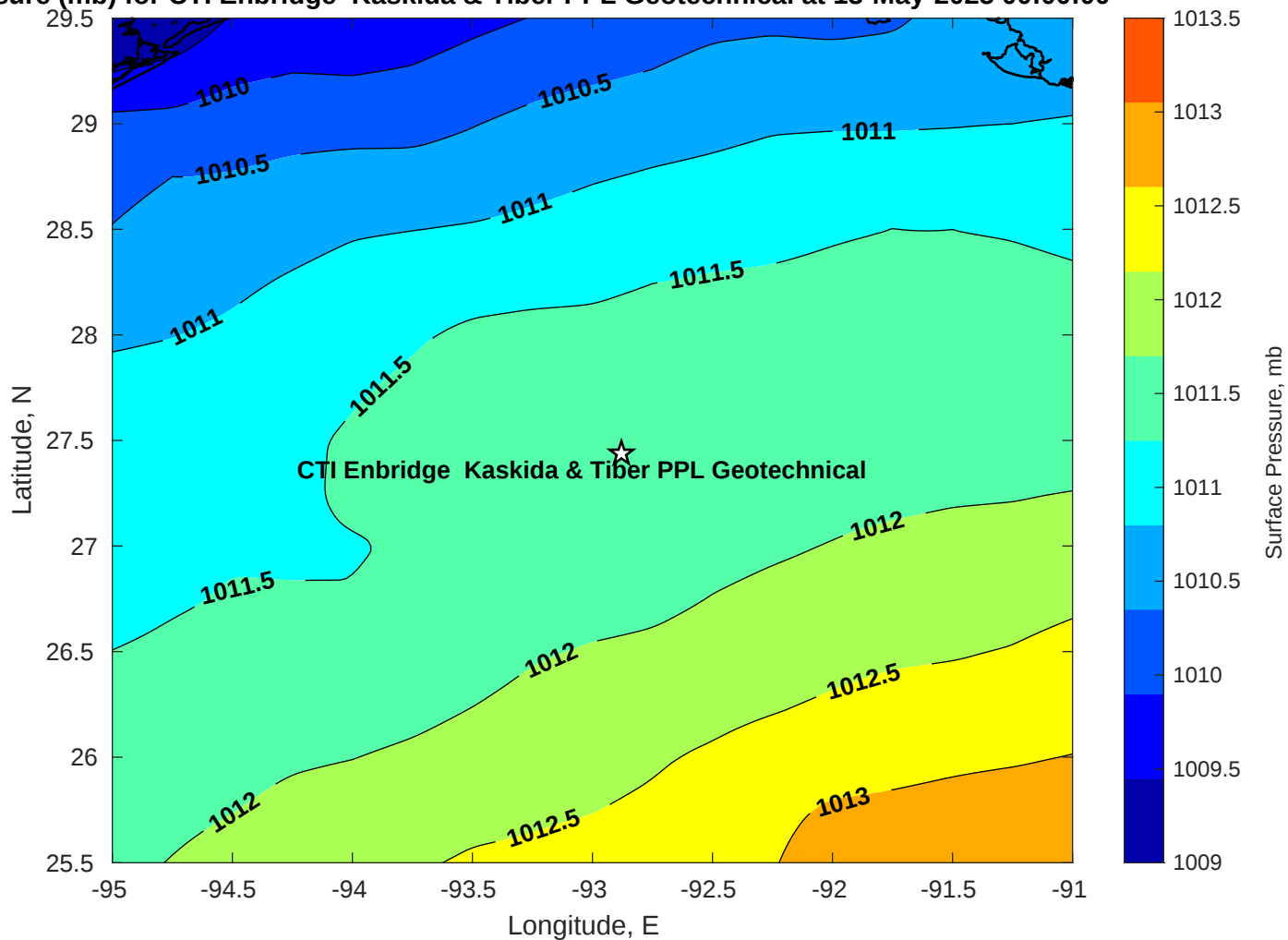
Surface Pressure (mb) for CTI Enbridge Kaskida & Tiber PPL Geotechnical at 13-May-2025 00:00:00
