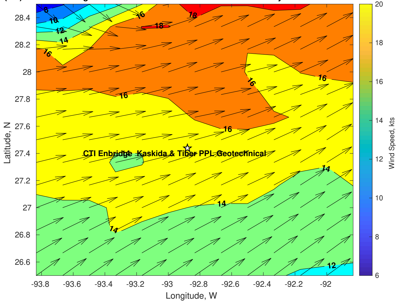
Winds (kts) for CTI Enbridge Kaskida & Tiber PPL Geotechnical at 12-May-2025 09:00:00
