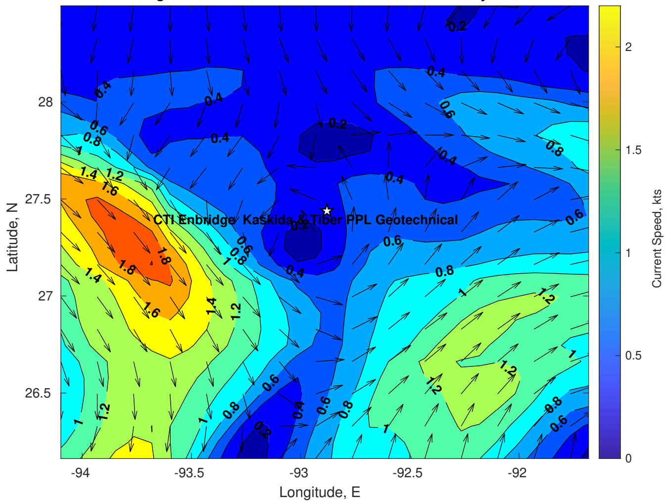
Surface Currents for CTI Enbridge Kaskida & Tiber PPL Geotechnical at 11-May-2025 00:00:00
