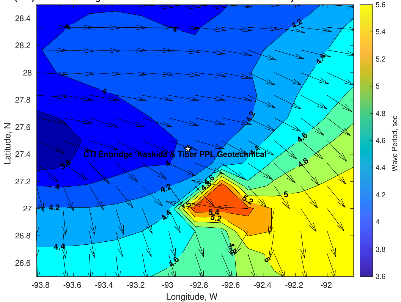
Wave Period (sec) for CTI Enbridge Kaskida & Tiber PPL Geotechnical at 12-May-2025 09:00:00
