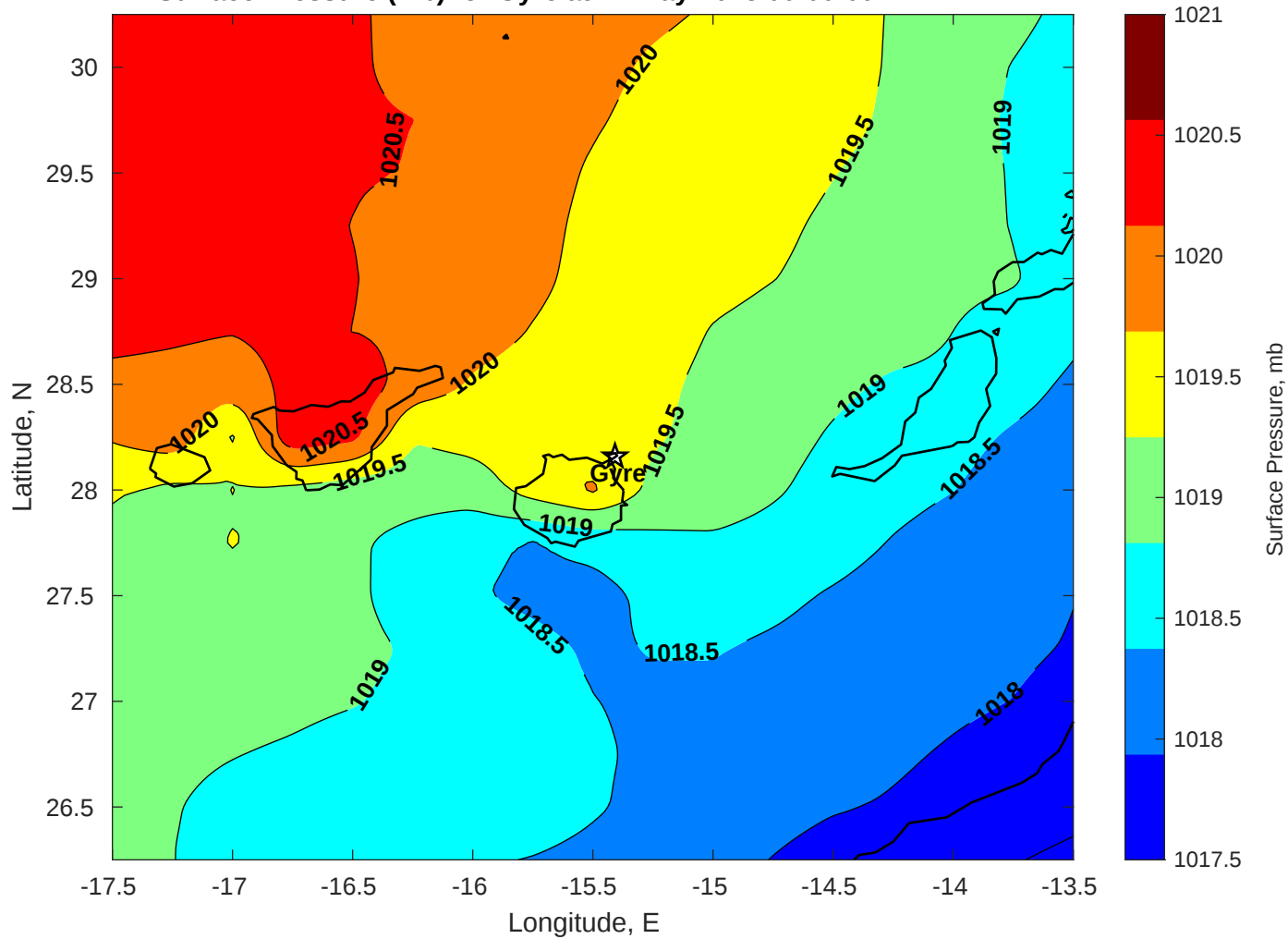
Surface Pressure (mb) for Gyre at 14-May-2025 00:00:00
