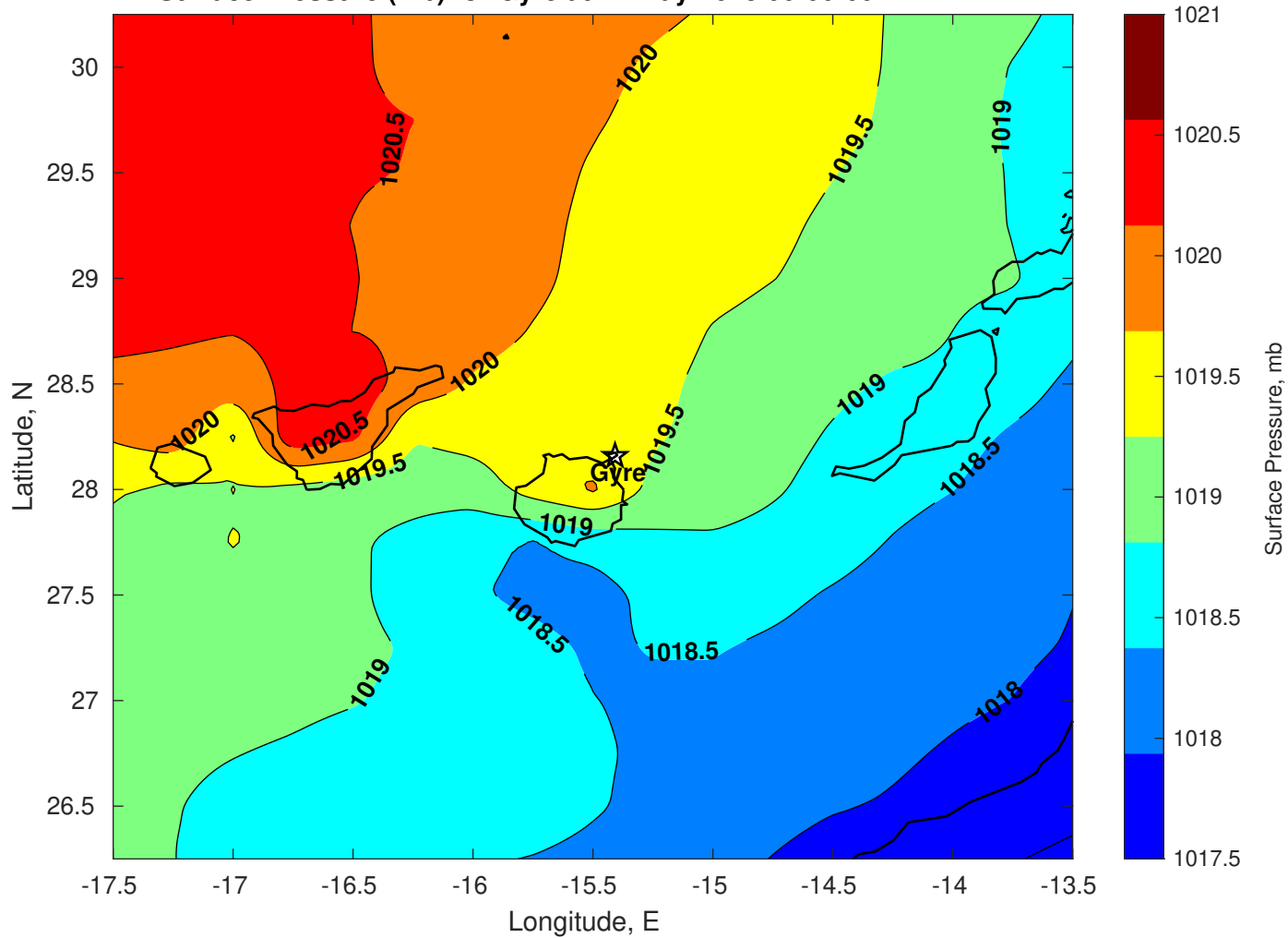
Surface Pressure (mb) for Gyre at 14-May-2025 00:00:00
