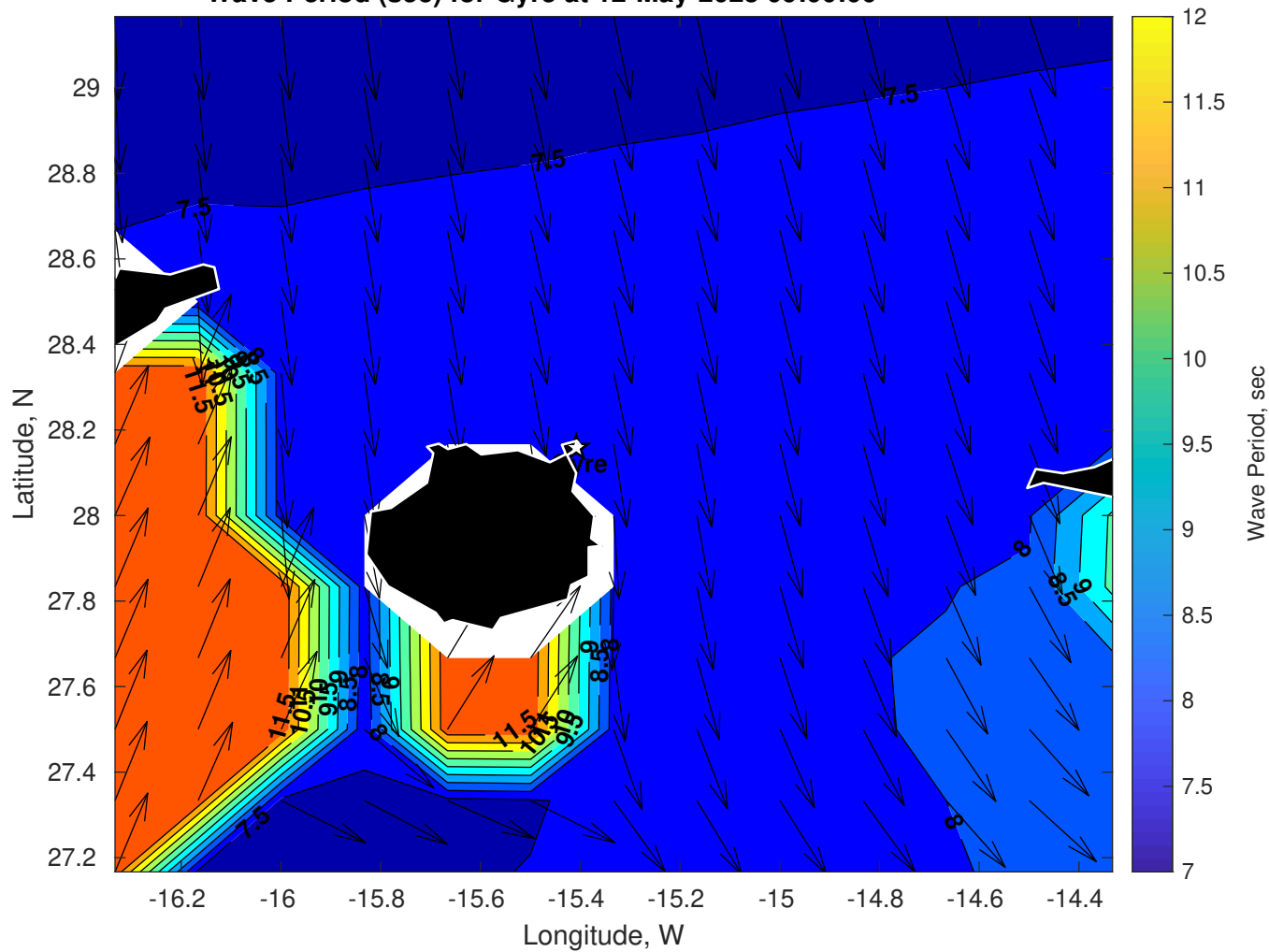
Wave Period (sec) for Gyre at 12-May-2025 09:00:00
