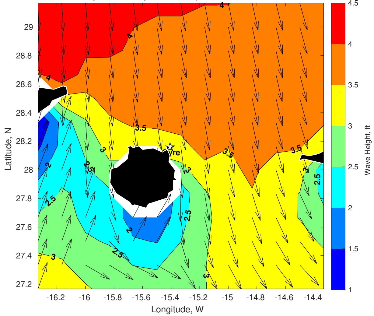
Wave Height (ft) for Gyre at 12-May-2025 09:00:00
