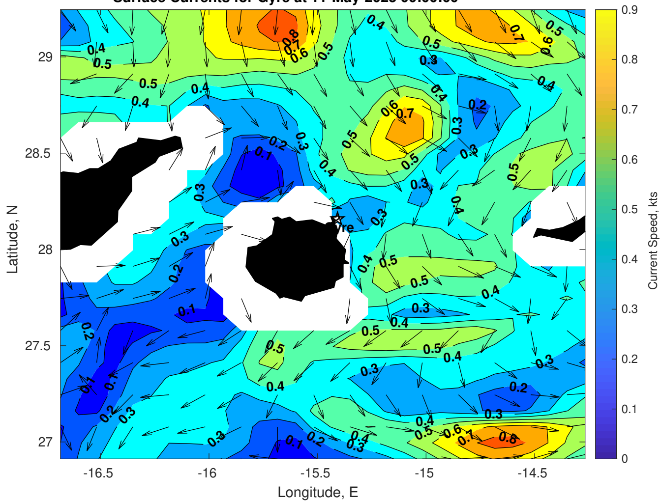
Surface Currents for Gyre at 11-May-2025 00:00:00
