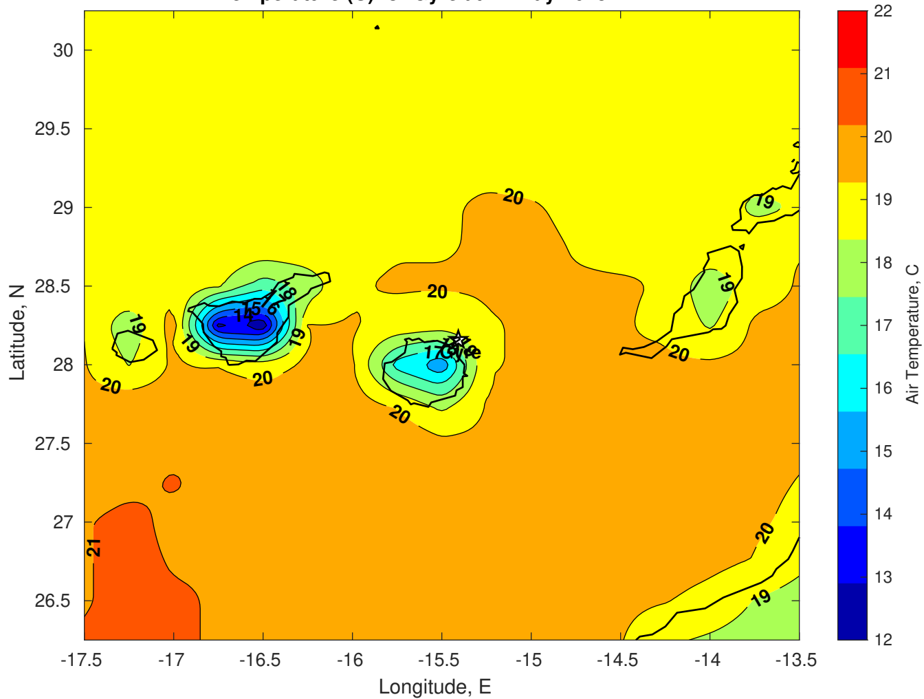
Air Temperature (C) for Gyre at 12-May-2025
