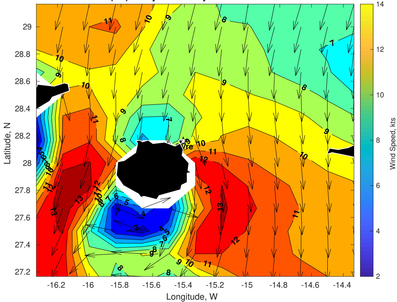
Winds (kts) for Gyre at 12-May-2025 09:00:00
