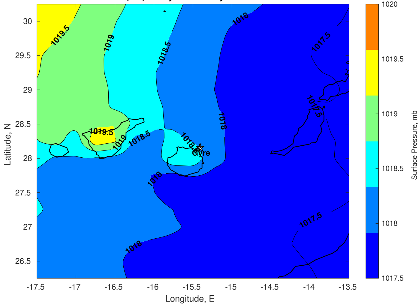
Surface Pressure (mb) for Gyre at 12-May-2025 00:00:00
