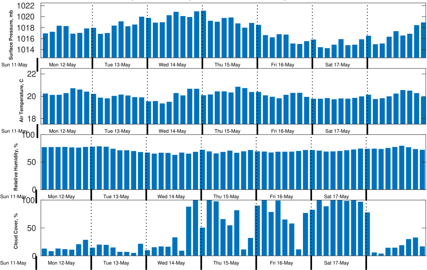
Met Forecast for Gyre from 11-May-2025 23:00:00 to 18-May-2025 23:00:00
