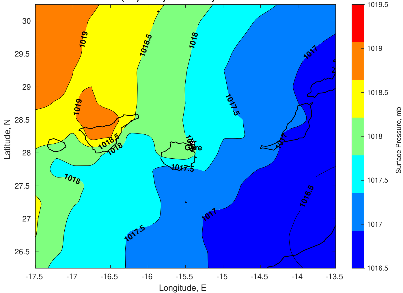
Surface Pressure (mb) for Gyre at 13-May-2025 00:00:00
