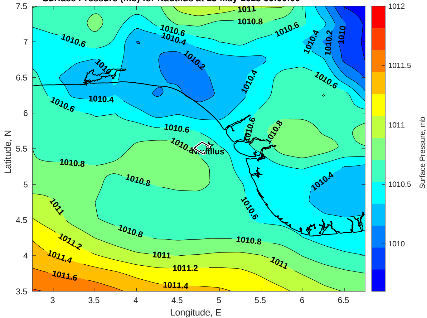
Surface Pressure (mb) for Nautilus at 13-May-2025 00:00:00
