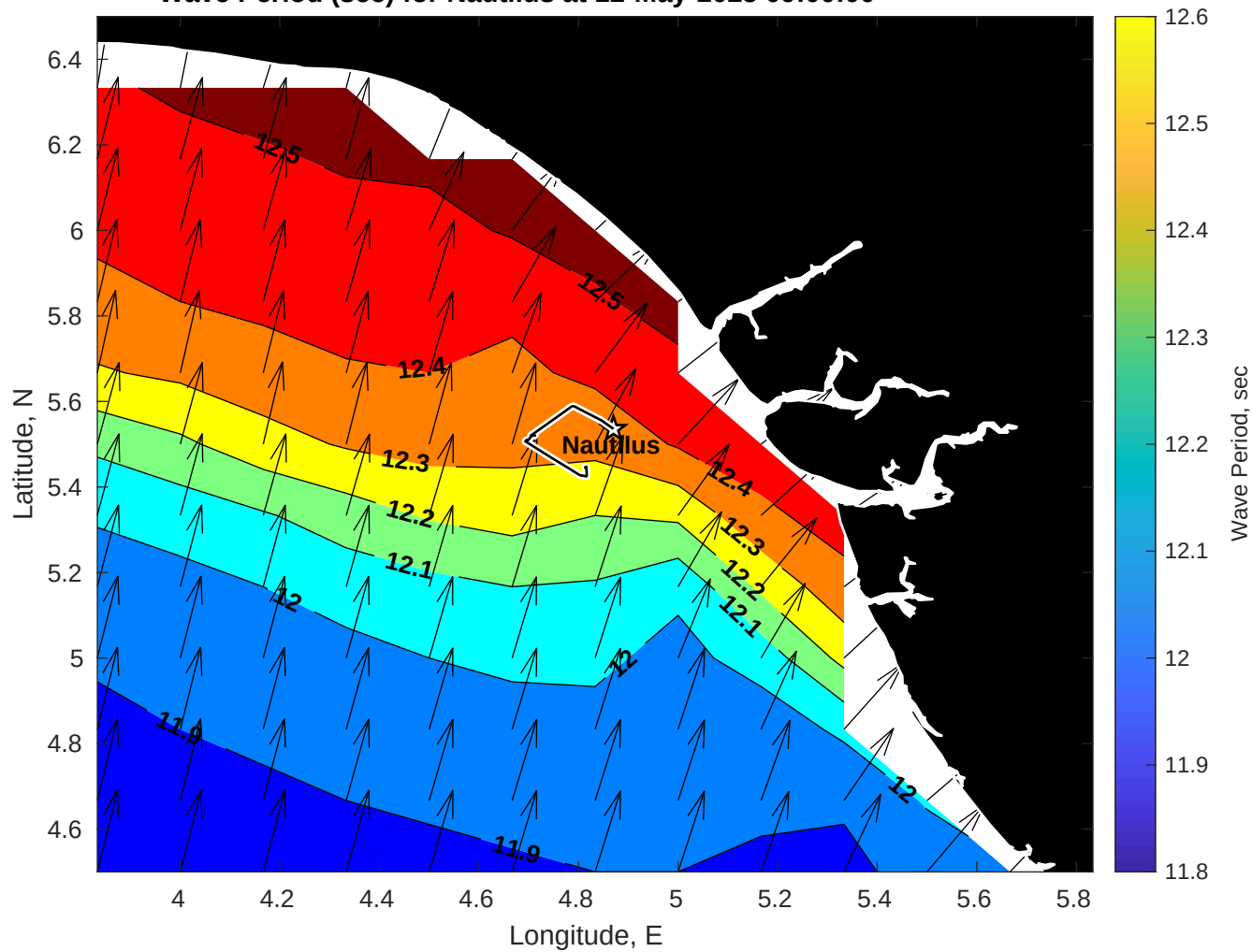
Wave Period (sec) for Nautilus at 12-May-2025 09:00:00
