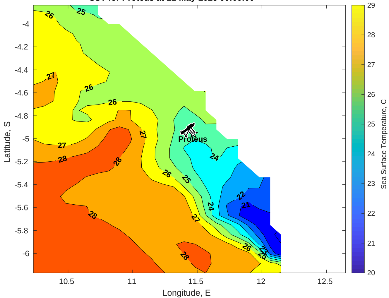
SST for Proteus at 11-May-2025 00:00:00
