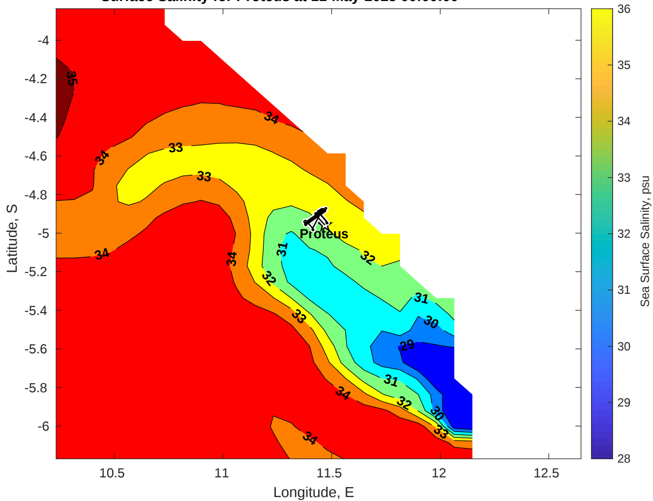
Surface Salinity for Proteus at 11-May-2025 00:00:00
