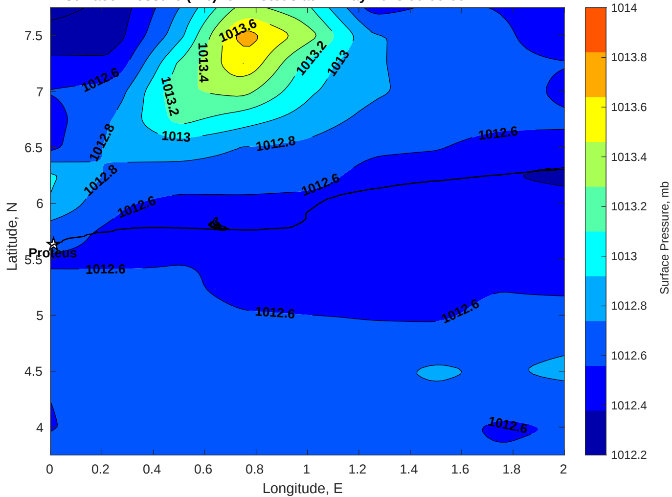
Surface Pressure (mb) for Proteus at 12-May-2025 00:00:00
