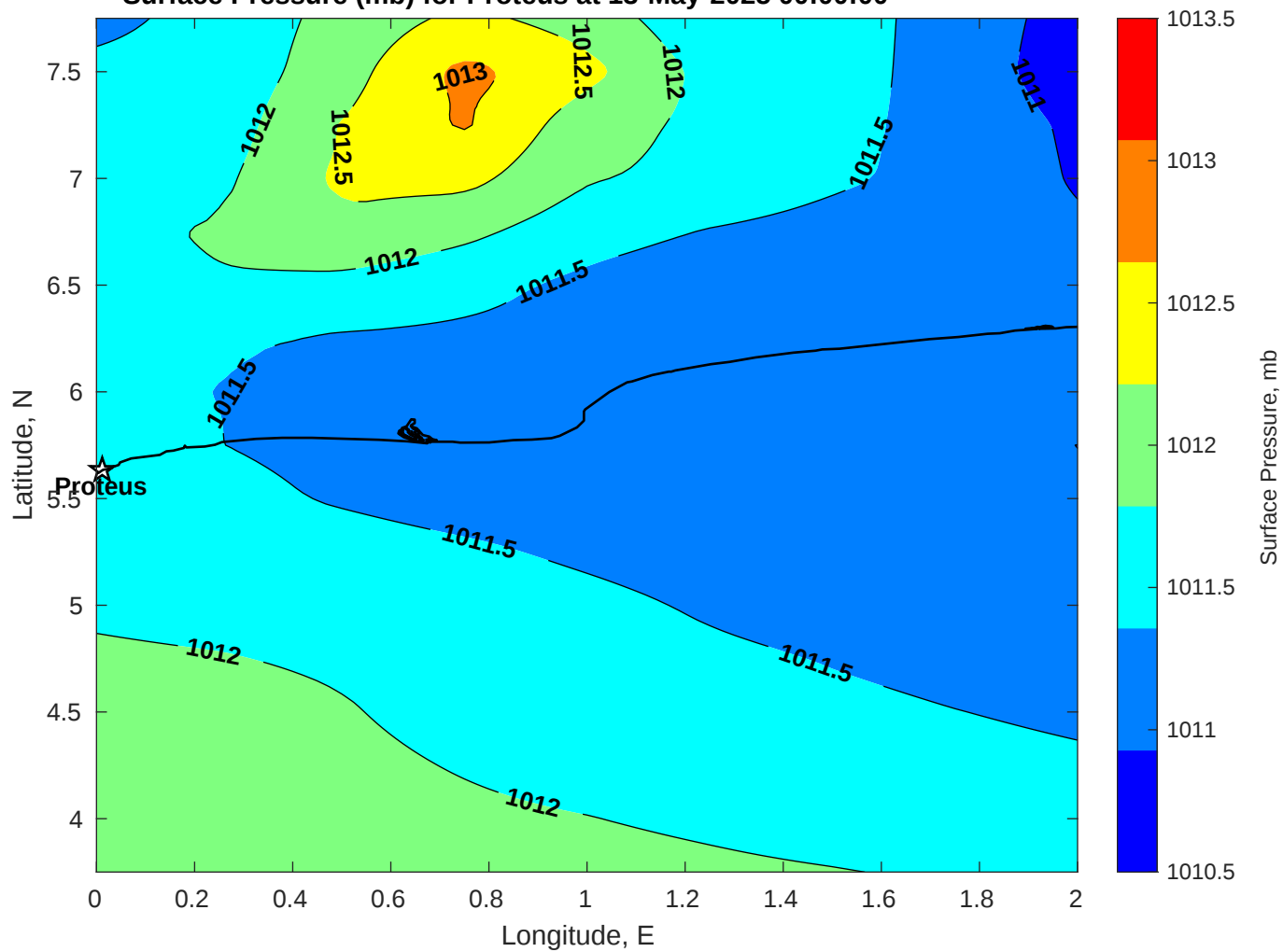
Surface Pressure (mb) for Proteus at 13-May-2025 00:00:00
