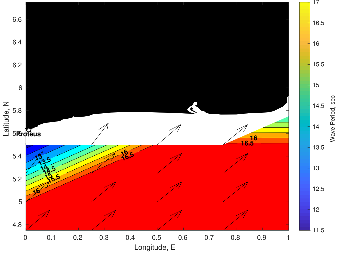
Wave Period (sec) for Proteus at 12-May-2025 09:00:00
