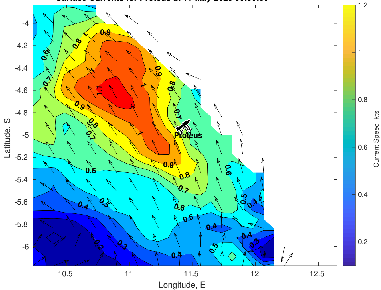
Surface Currents for Proteus at 11-May-2025 00:00:00
