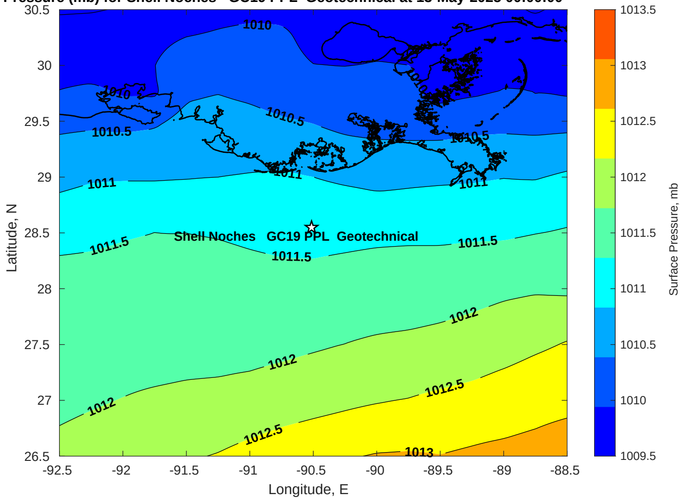
Surface Pressure (mb) for Shell Noches GC19 PPL Geotechnical at 13-May-2025 00:00:00
