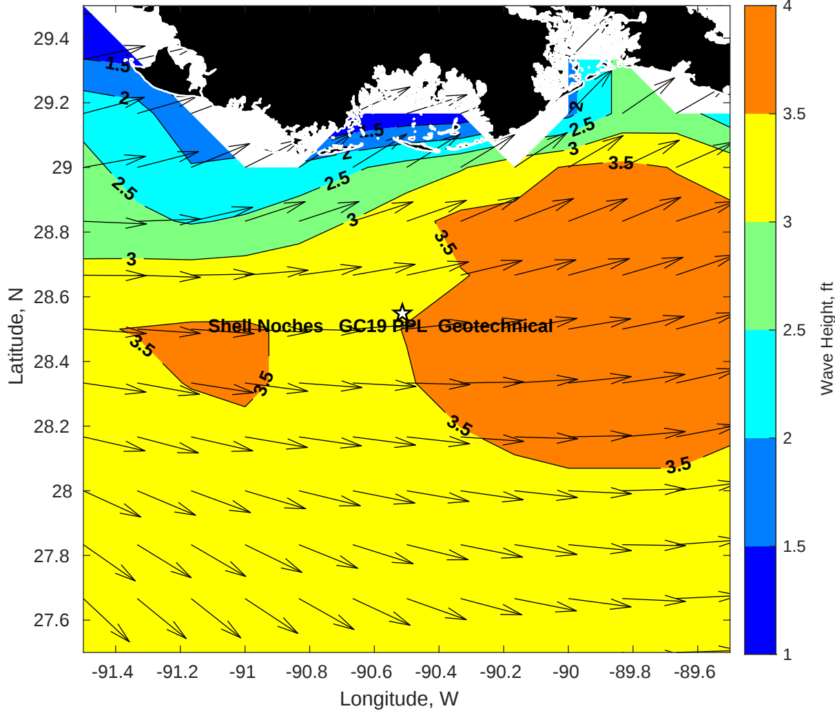
Wave Height (ft) for Shell Noches GC19 PPL Geotechnical at 12-May-2025 09:00:00
