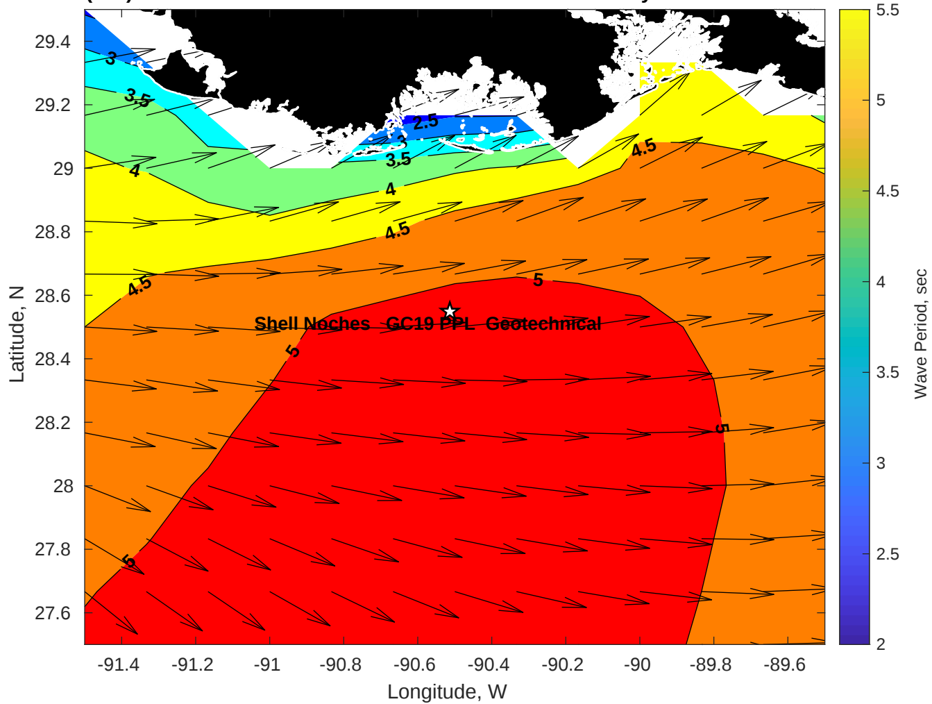
Wave Period (sec) for Shell Noches GC19 PPL Geotechnical at 12-May-2025 09:00:00
