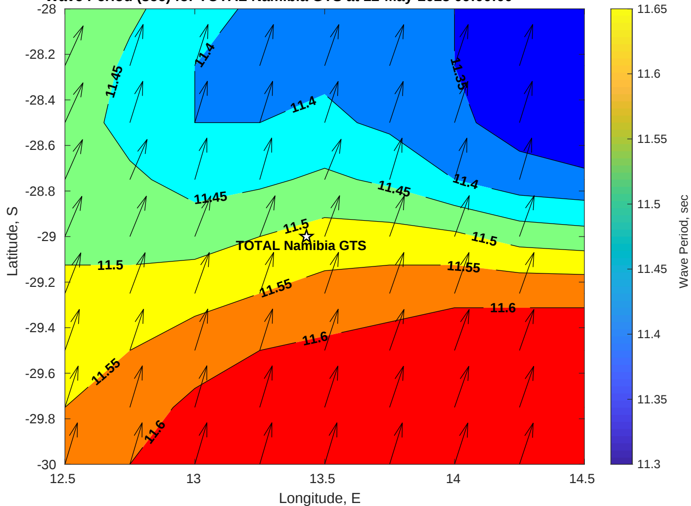
Wave Period (sec) for TOTAL Namibia GTS at 12-May-2025 09:00:00
