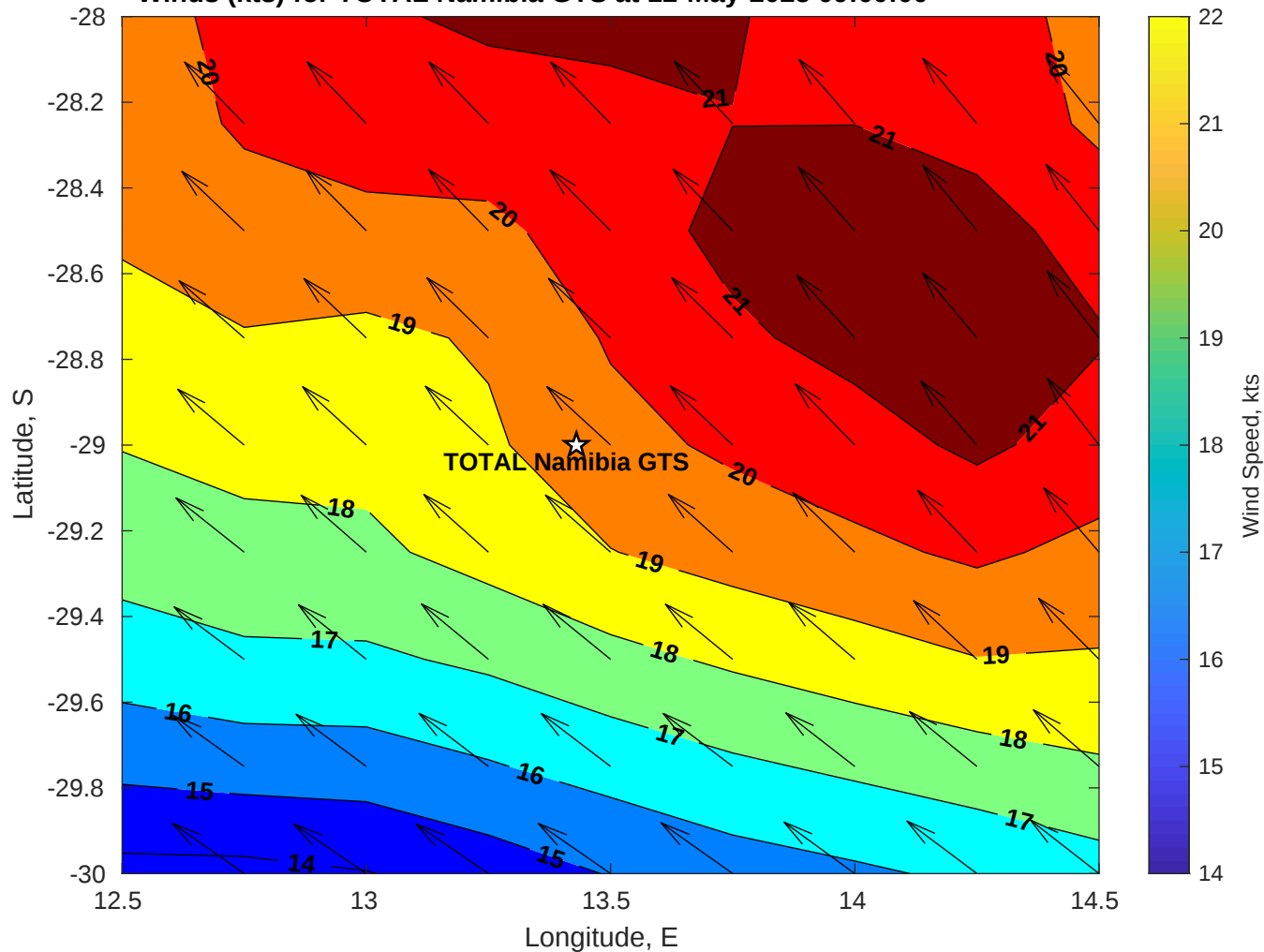
Winds (kts) for TOTAL Namibia GTS at 12-May-2025 09:00:00
