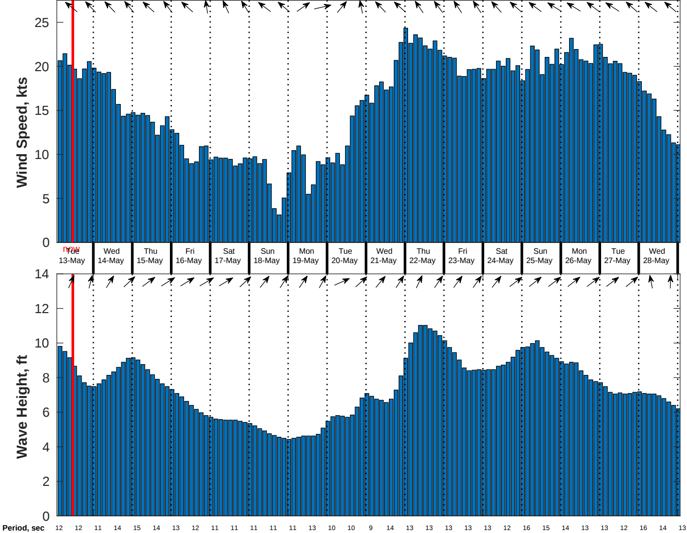
Wind & Wave Forecast for TOTAL Namibia GTS from 12-May-2025 02:00:00 to 28-May-2025 02:00:00
