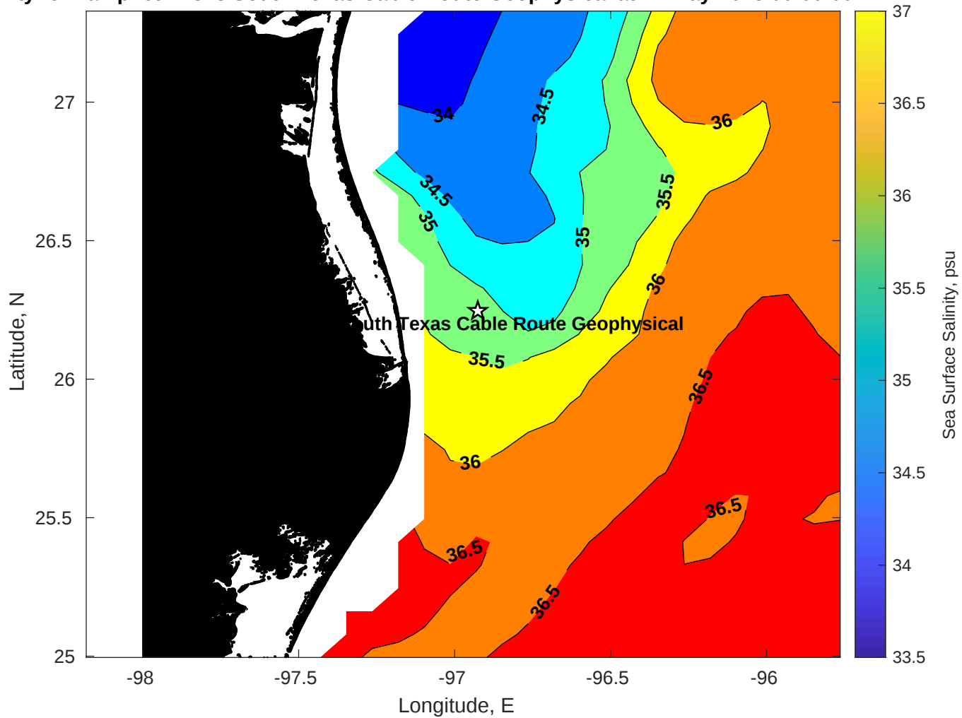
Surface Salinity for Tampnet P2378 South Texas Cable Route Geophysical at 11-May-2025 00:00:00
