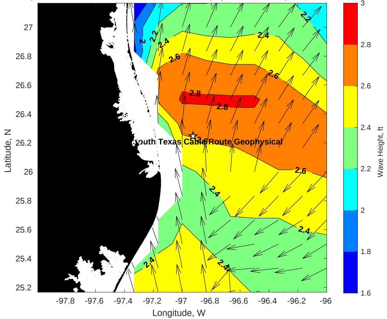
Wave Height (ft) for Tampnet P2378 South Texas Cable Route Geophysical at 12-May-2025 09:00:00
