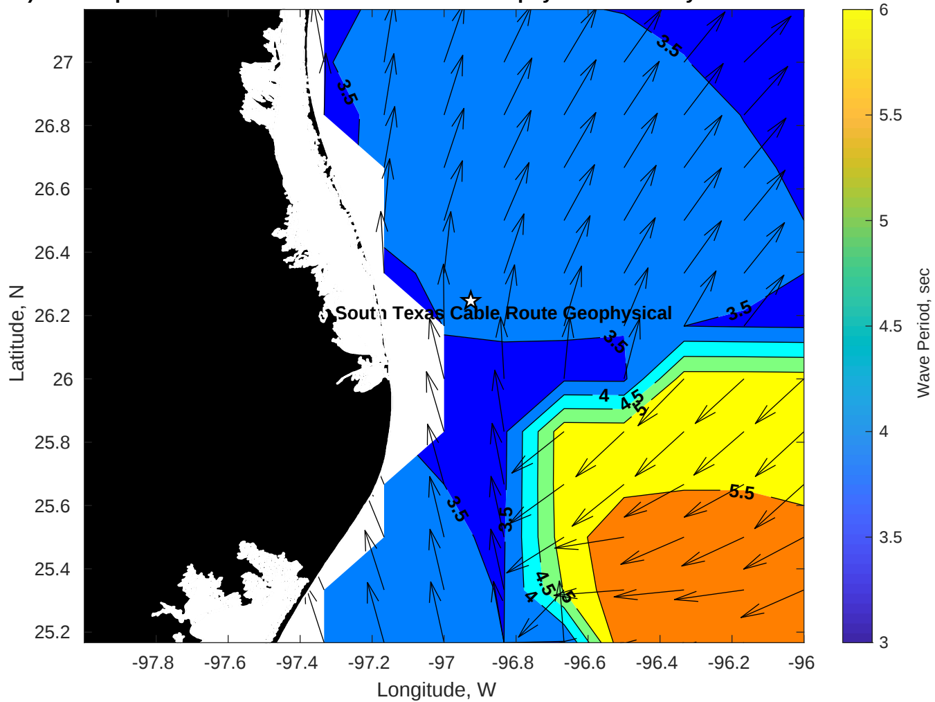
Period (sec) for Tampnet P2378 South Texas Cable Route Geophysical at 12-May-2025 09:00:00
